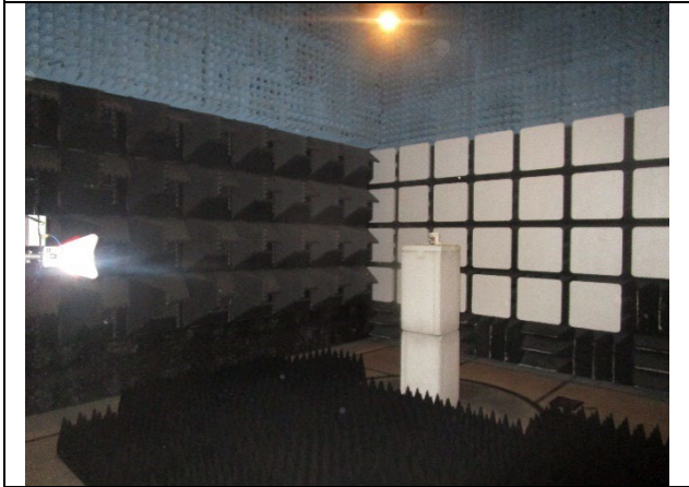
Radiated Emissions 1000-25000 MHz
