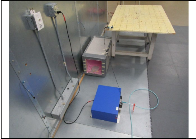
AC Conducted Emissions
