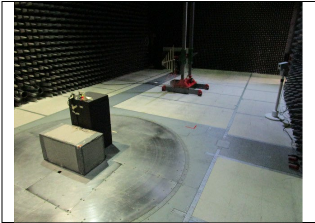
Radiated Emissions 30-1000 MHz
