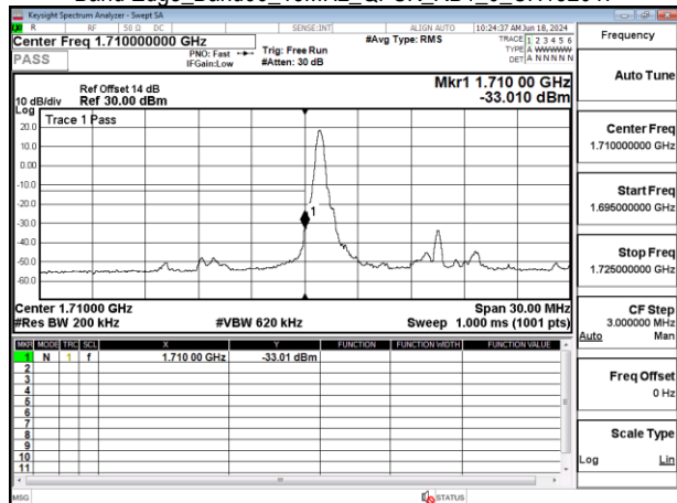
Band Edge_Band66_15MHz_QPSK_RB1_74_CH132597
