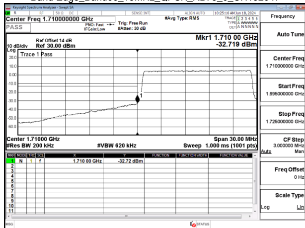
Band Edge_Band66_15MHz_QPSK_RB75_0_CH132047
