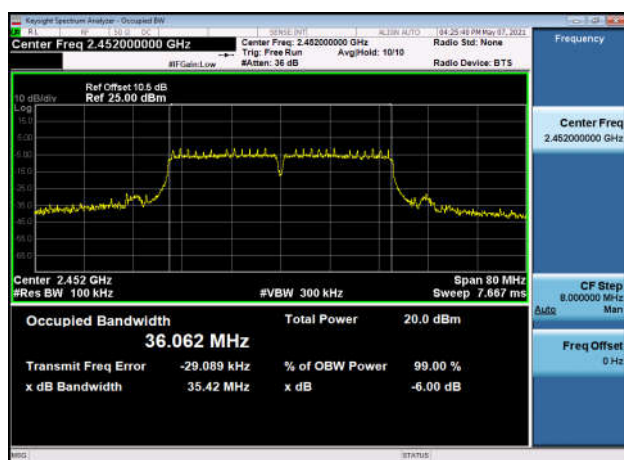
6dB Bandwidth-802.11n(HT40),2452MHz
