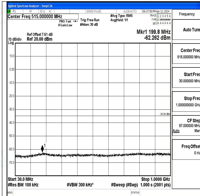
Band7_20MHz_QPSK_20850_1RB#0_30~1000_30~100 0
