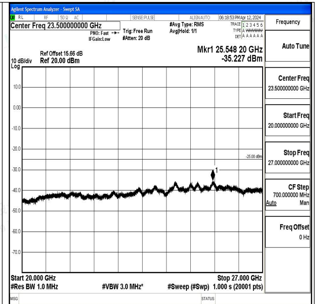
Band7_15MHz_16QAM_21375_1RB#0_20000~27000_2 0000~27000
