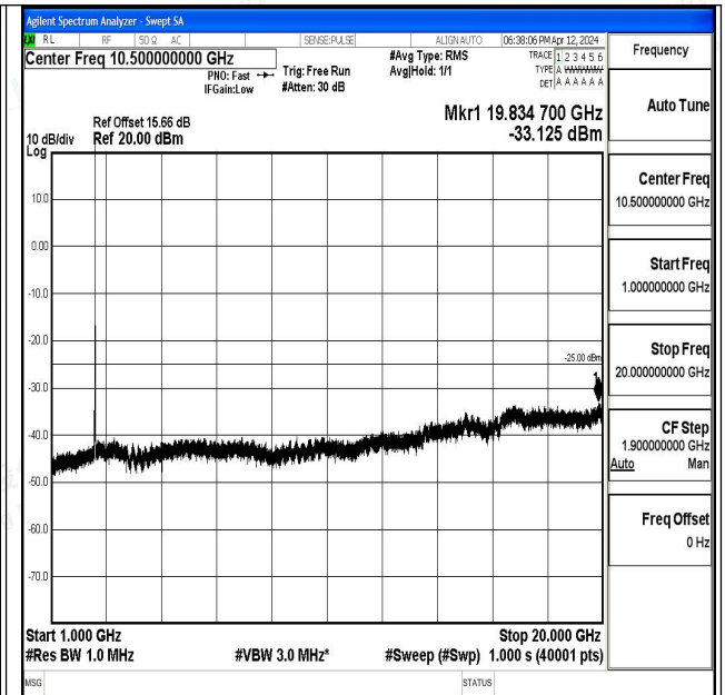
Band7_20MHz_QPSK_20850_1RB#0_1000~20000_100 0~20000
