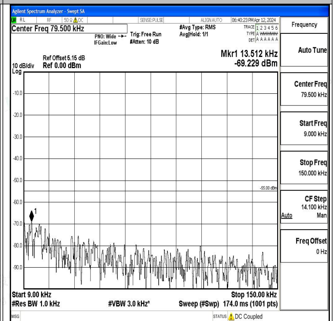
Band7_20MHz_16QAM_21350_1RB#0_0.009~0.15_0.0 09~0.15
