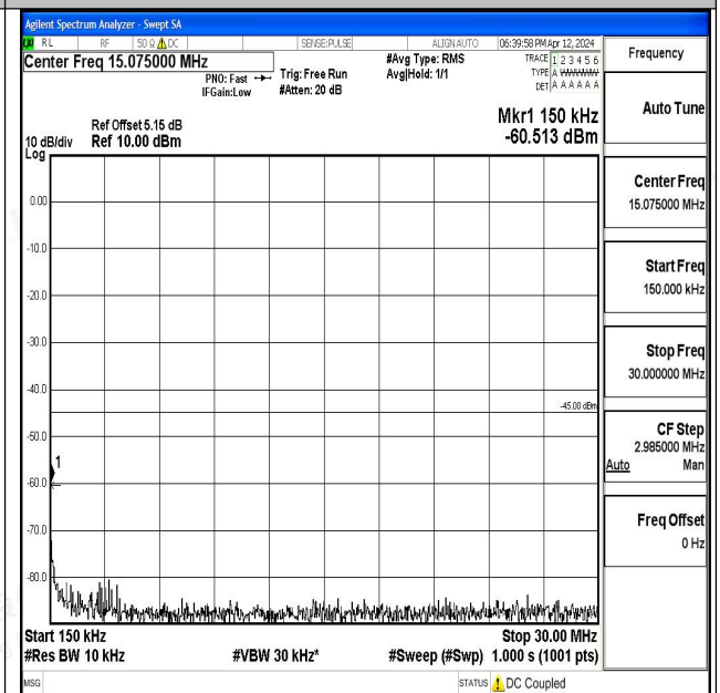
Band7_20MHz_QPSK_21350_1RB#0_0.15~30_0.15~30
