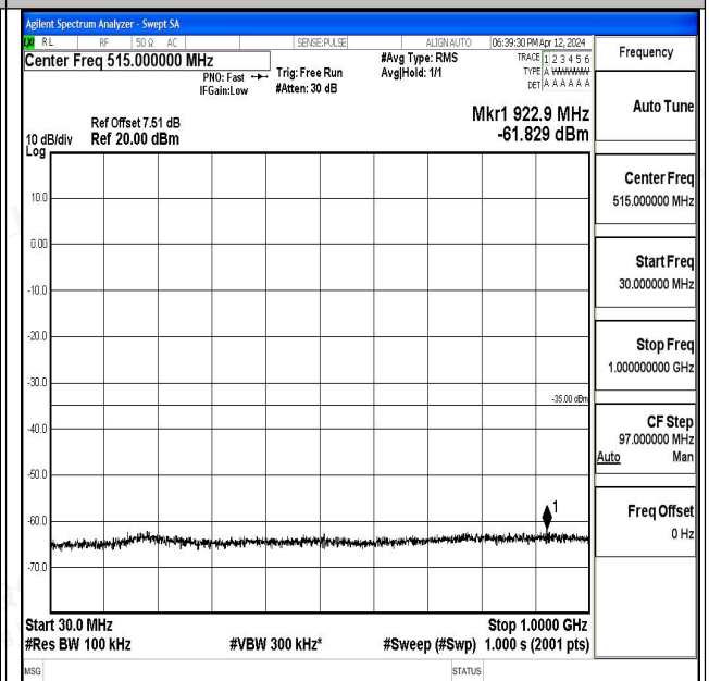
Band7_20MHz_16QAM_21100_1RB#0_30~1000_30~10 00
