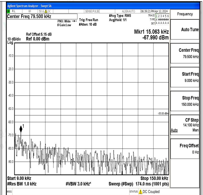
Band7_20MHz_16QAM_21100_1RB#0_0.009~0.15_0.00 9~0.15
