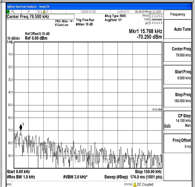
Band7_20MHz_16QAM_20850_1RB#0_0.009~0.15_0.0 09~0.15
