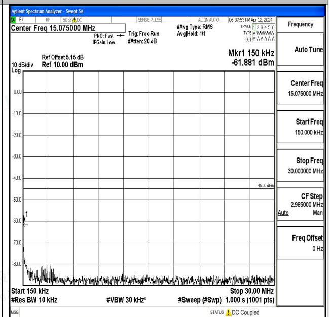
Band7_20MHz_QPSK_20850_1RB#0_0.15~30_0.15~30
