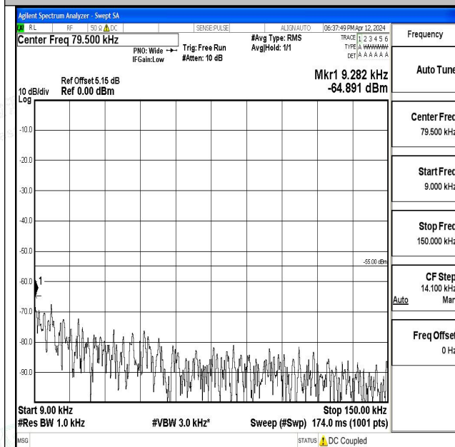
Band7_20MHz_QPSK_20850_1RB#0_0.009~0.15_0.009 ~0.15
