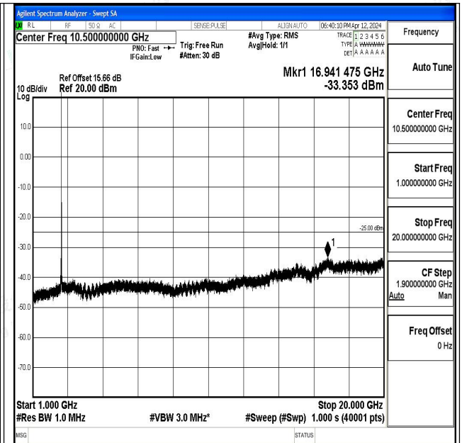
Band7_20MHz_QPSK_21350_1RB#0_1000~20000_100 0~20000
