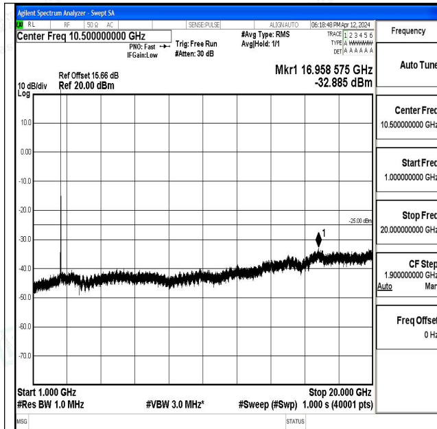
Band7_15MHz_16QAM_21375_1RB#0_1000~20000_10 00~20000
