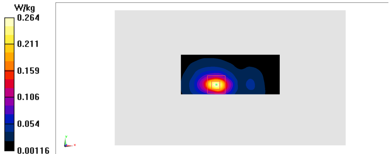
Fig.142450 MHz
