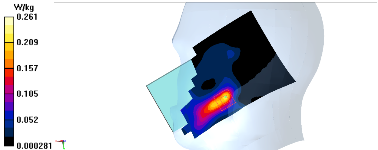
Fig.11 LTE Band 38
