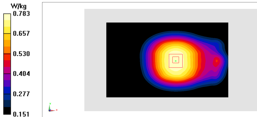
Fig.2 850 MHz
