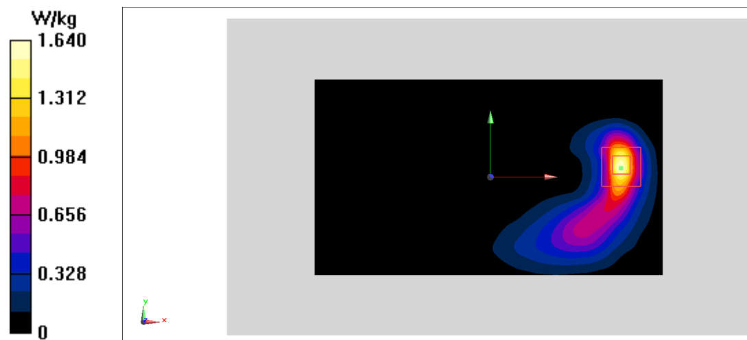
Fig.12 LTE Band 38
