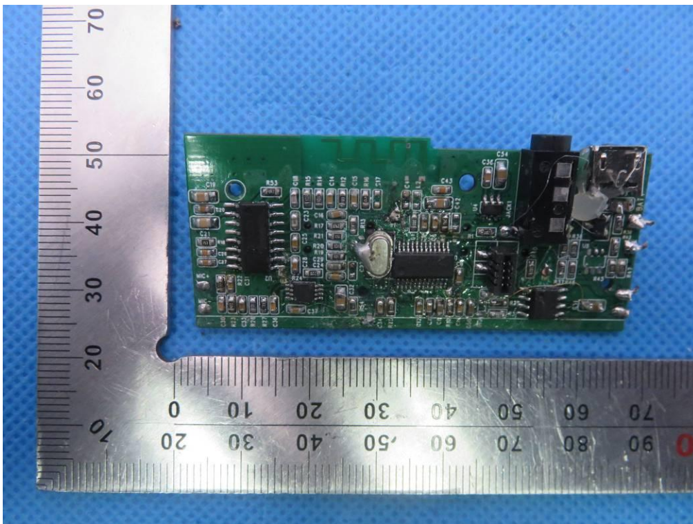
SERIES MODEL-SMM465B INTERNAL VIEW OF EUT-1
