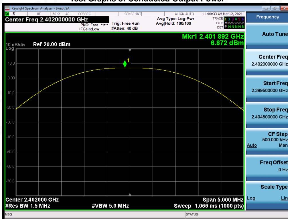
Test_Graph_LE1M_2402_1Mbps_Peak Power
