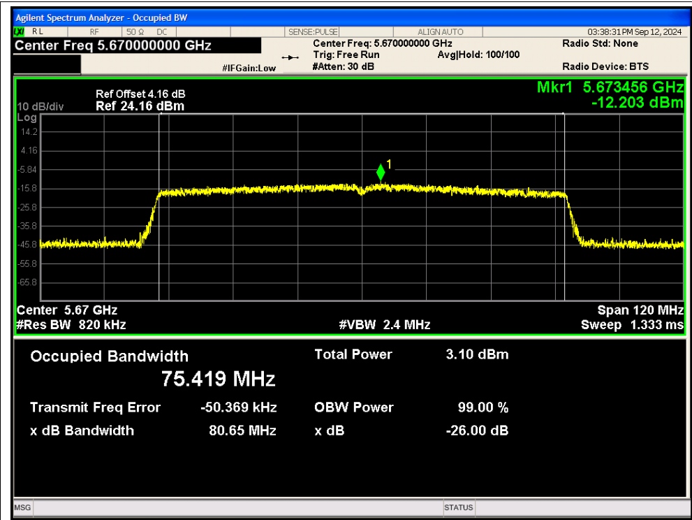
OBW NVNT ac80 5670MHz Ant2
