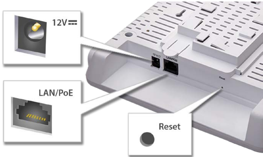
Figure 2-2 Rear Panel of C-65
