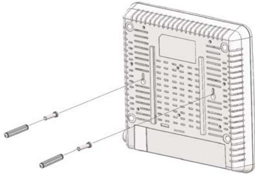
Figure 3-2 Wall Mounting
