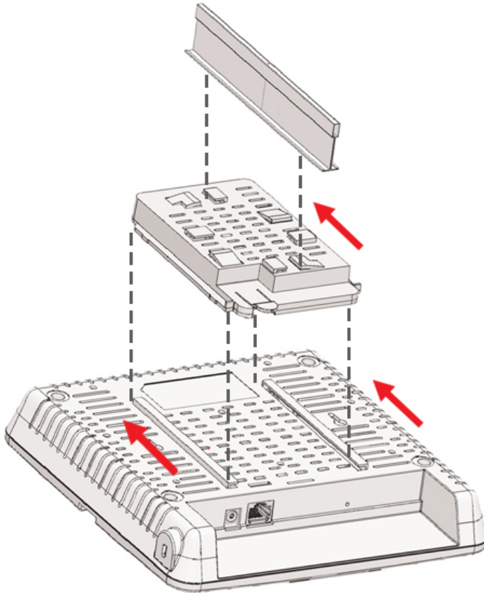
Figure 3-1 Ceiling Mounting
