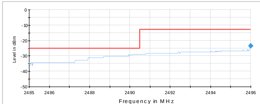
030420_BandEdge_Low_FCC_Part27_LTE7_All-Channels_nokipp
