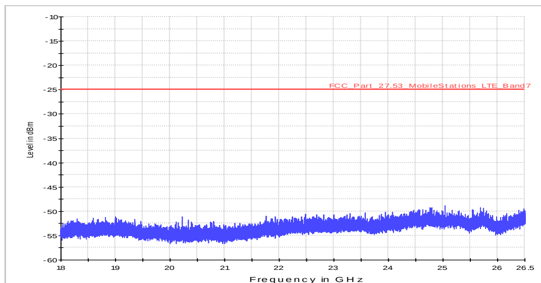
Fula2_FCC_Part27_LTE_Bd7_18_26.5GHz_Peak
