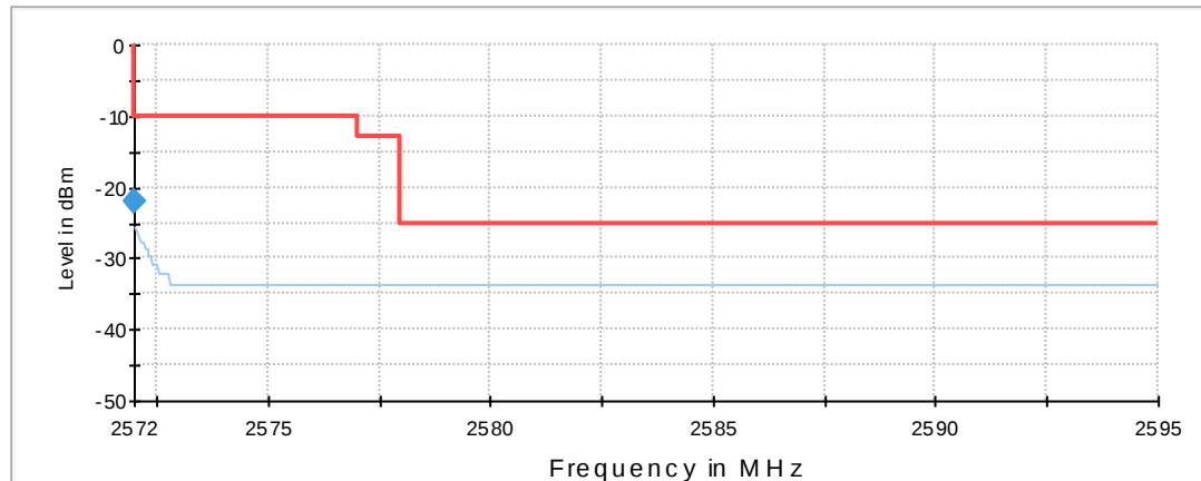
030420_BandEdge_High_FCC_Part27_LTE7_All-Channels_nokipp
