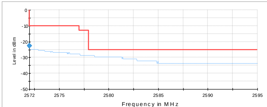
030420_BandEdge_High_FCC_Part27_LTE7_All-Channels_nokipp
