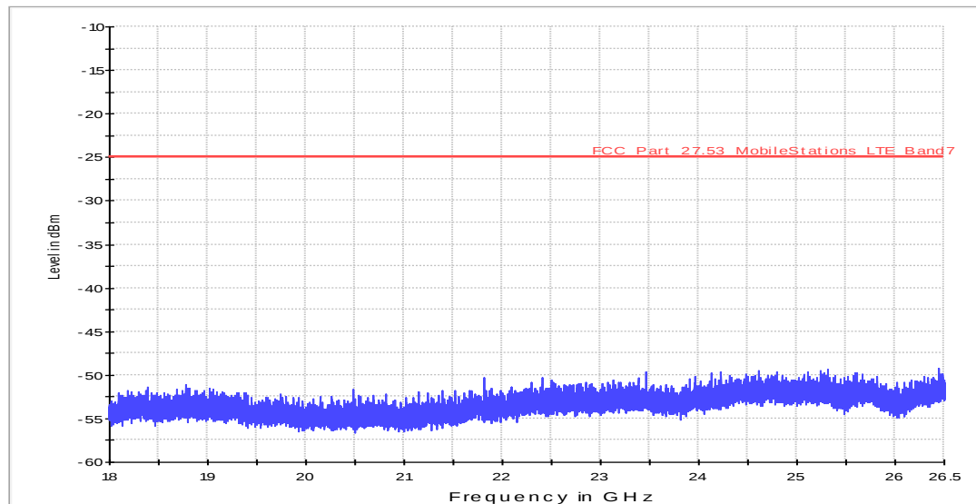
Fula2_FCC_Part27_LTE_Bd7_18_26.5GHz_Peak
