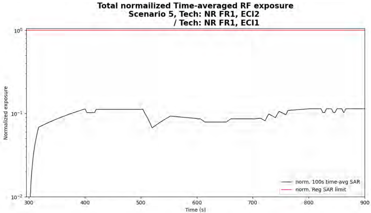
Figure 5- 47 Normalized time-averaged SAR for case 15 (sub6 FR1 B66(Lower))
