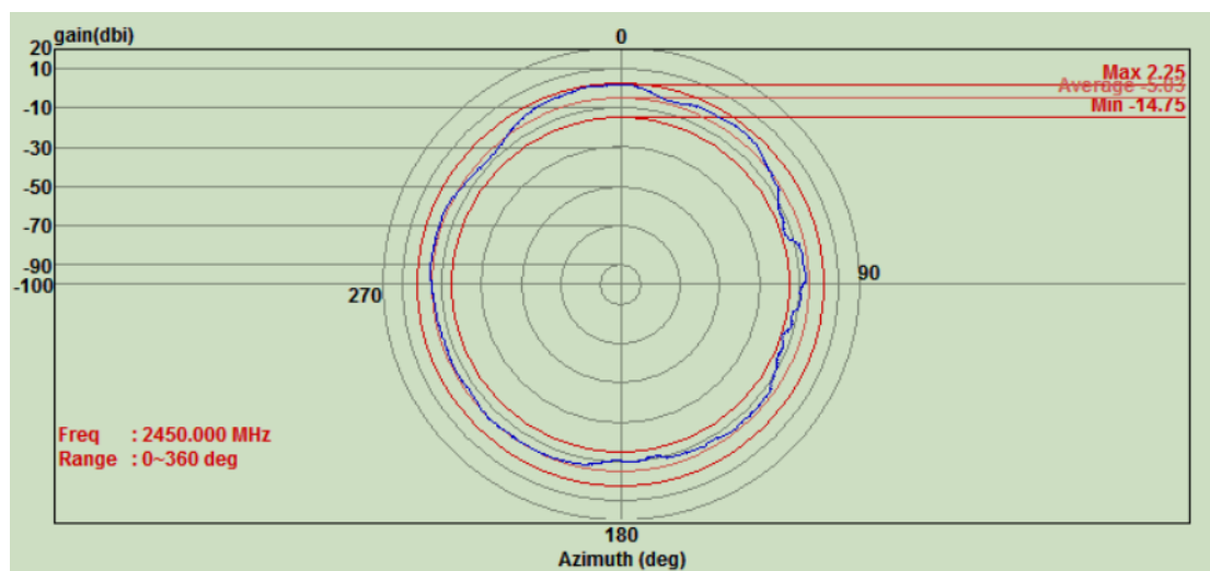
Figure3 Antenna ANT1, 2450MHz
