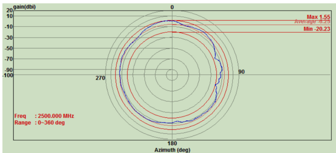
Figure4 Antenna ANT1, 2500MHz
