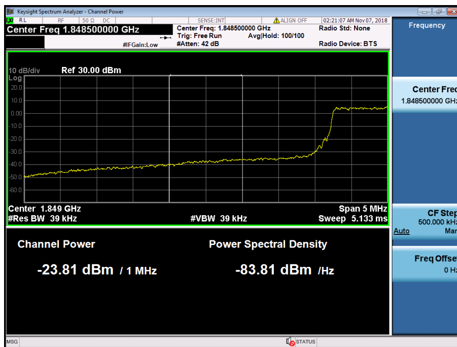
LTE Band 2 / 5MHz / 16QAM Offset/Size (12/0)
