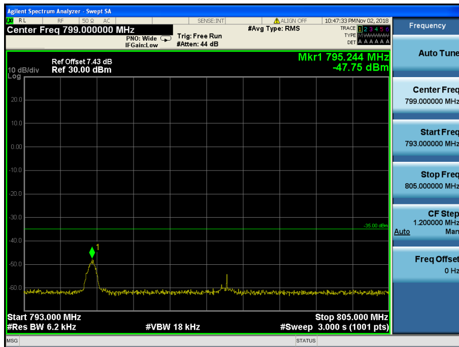
LTE Band 13 / 10MHz / QPSK - RB Size/Offset (1/49)
