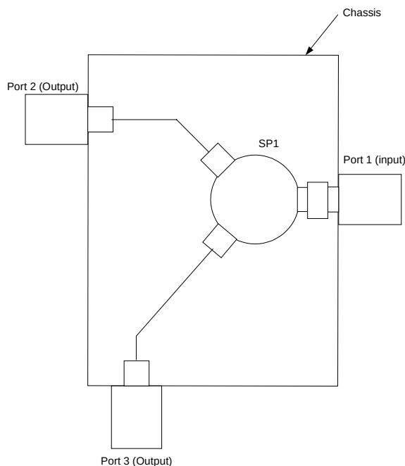
Figure 5-2 Calibration Splitter Box
