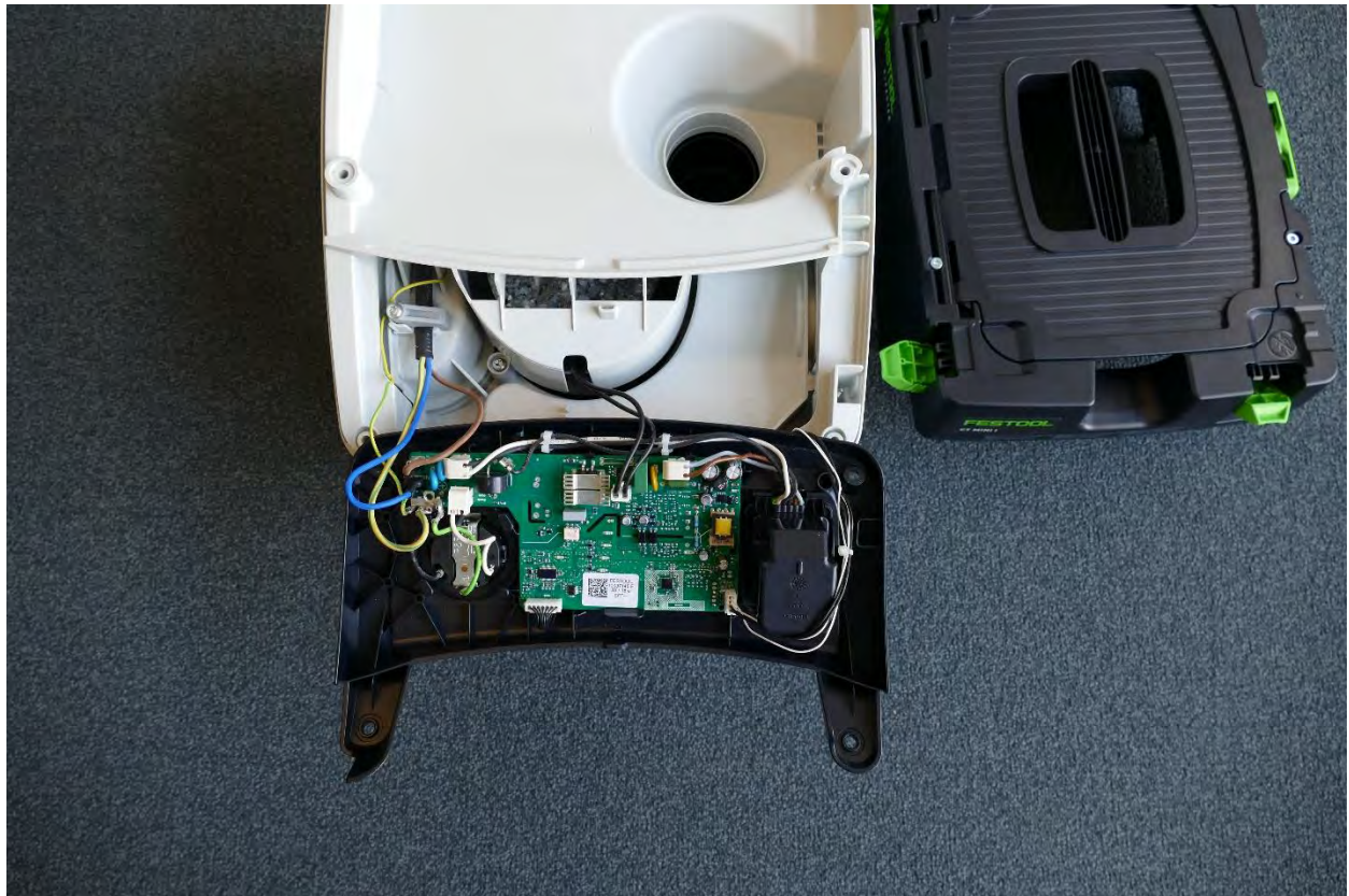
Front removed; board exposed
