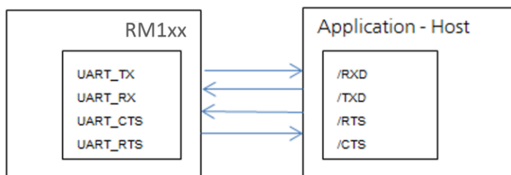
Figure 4: UART Signals
