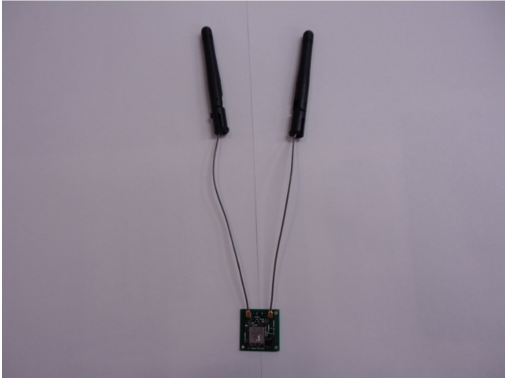
Antenna 1: Sleeve antenna
