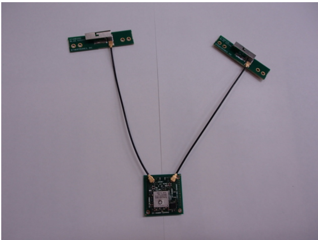
Antenna 2: Embedded antenna
