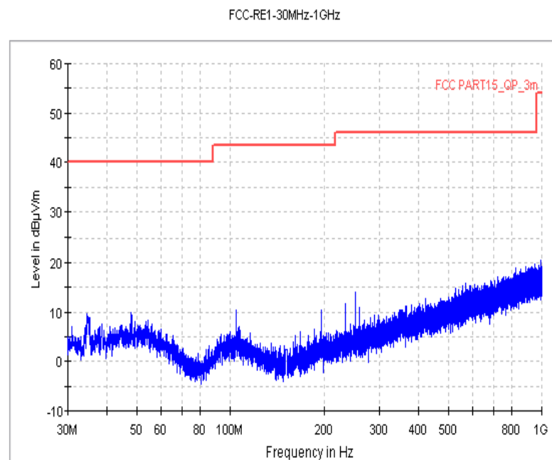
Fig.24 Radiated Spurious Emission (GFSK, Ch0, 30 MHz ~1 GHz, AE1)
