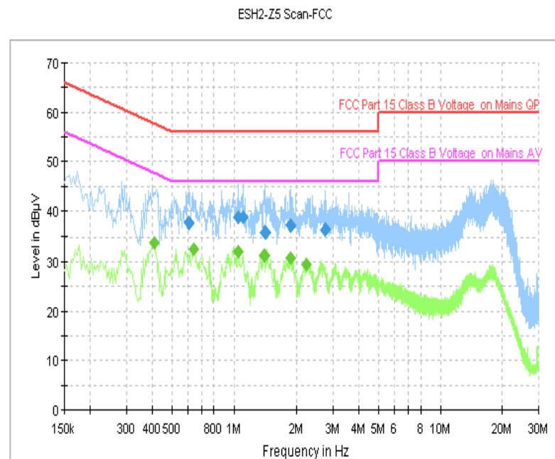
Fig. 31 AC Power line Conducted Emission (Idle, AE1)
