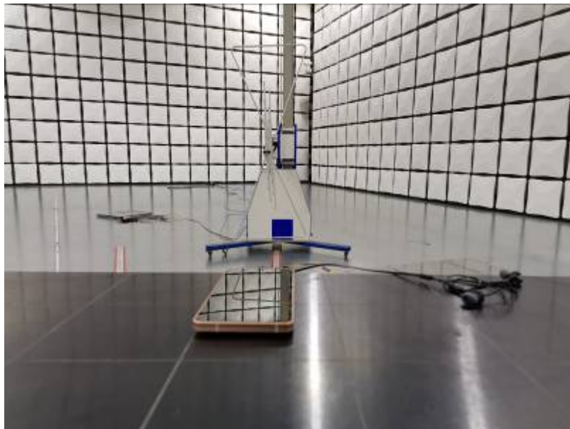
Radiated Emissions Test Setup (30-1000MHz)
