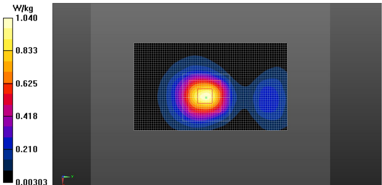
Fig.18 LTE Band 7
