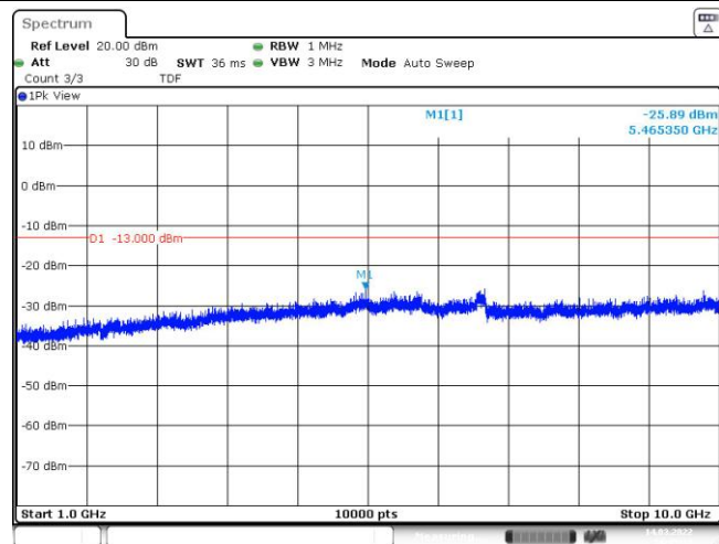
Band5-5MHz-16QAM-20425-25RB#0-Range2:1000~10000MHz
