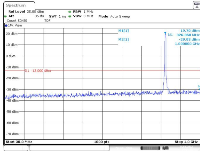
Band5-5MHz-16QAM-20425-25RB#0-Range1:30~1000MHz
