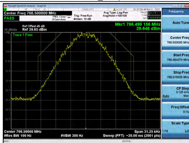
Pre-AGC_Output
