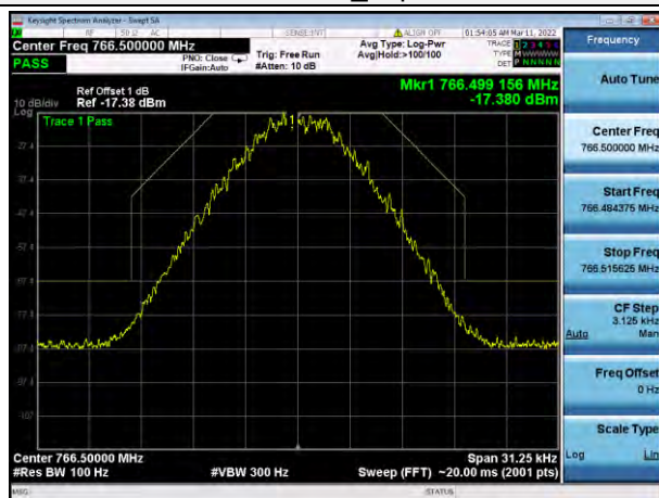
Pre-AGC_Input
