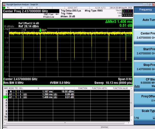
802.11g
