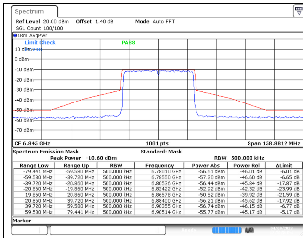
802.11ax (40MHz) 6845MHz Chain A NSS-4
