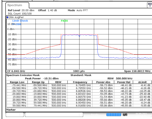
802.11ax (40MHz) 6845MHz Chain C NSS-4
