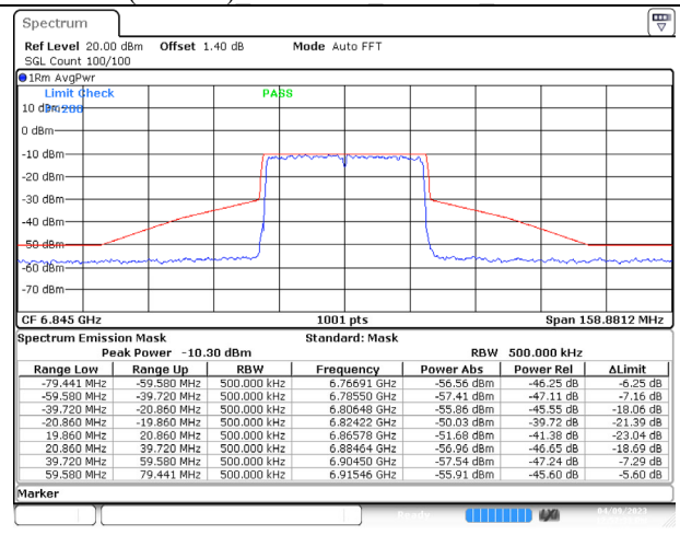
802.11ax (40MHz) 6845MHz Chain D NSS-4
