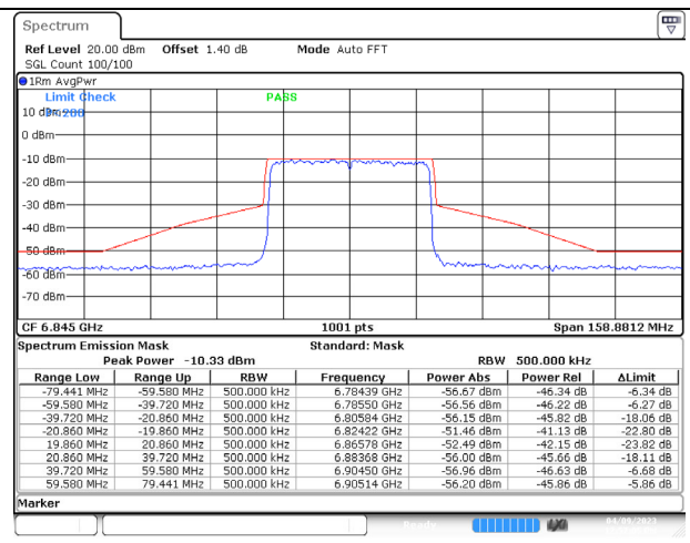
802.11ax (40MHz) 6845MHz Chain B NSS-4
