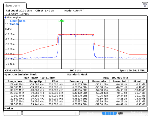
802.11ax (40MHz) 6445MHz Chain D NSS-4
