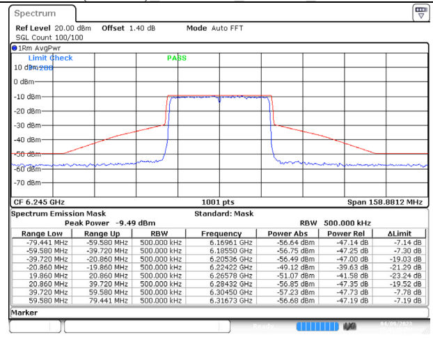
802.11ax (40MHz) 6245MHz Chain B NSS-4
