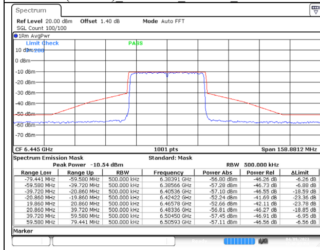
802.11ax (40MHz) 6445MHz Chain A NSS-4
