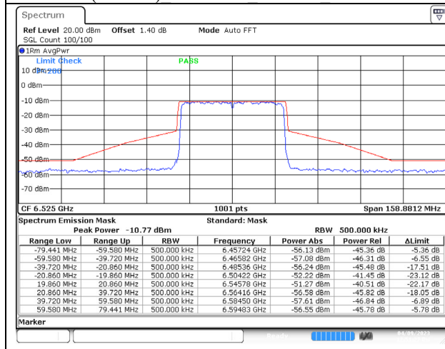
802.11ax (40MHz) 6525MHz Chain C NSS-4
