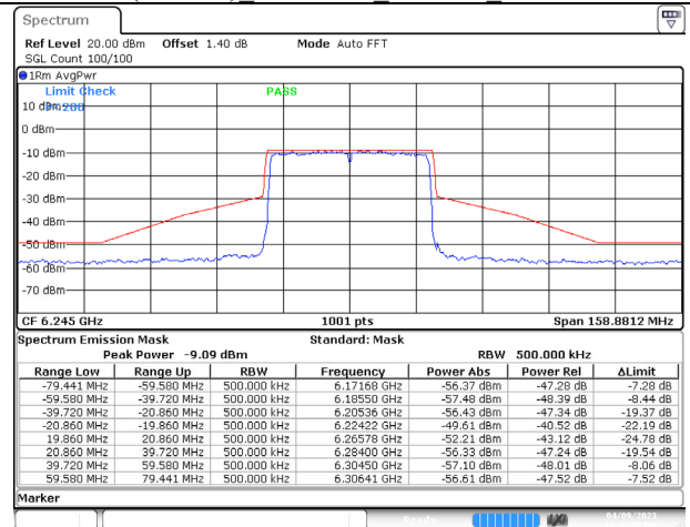
802.11ax (40MHz) 6245MHz Chain D NSS-4
