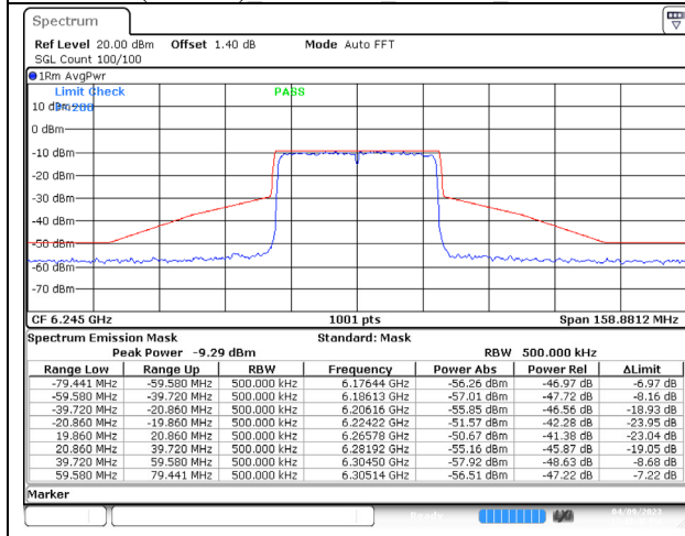
802.11ax (40MHz) 6245MHz Chain A NSS-4
