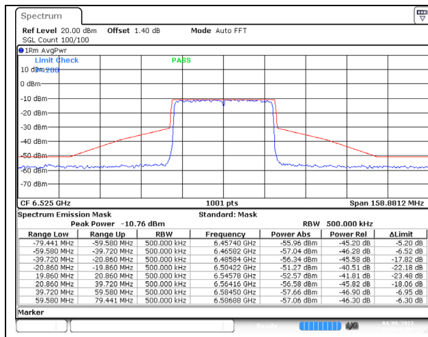
802.11ax (40MHz) 6525MHz Chain A NSS-4
