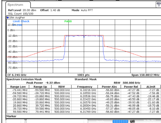
802.11ax (40MHz) 6245MHz Chain C NSS-4
