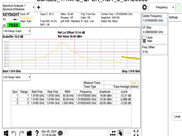
Band25_1.4MHz_QPSK_RB6_0_CH26683
