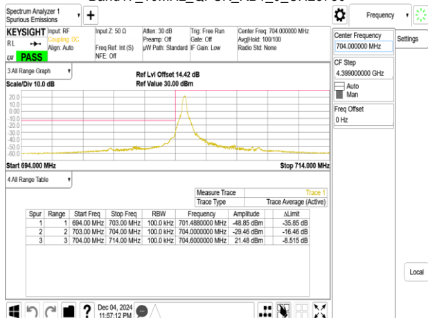
Band17_10MHz_QPSK_RB50_0_CH23780
