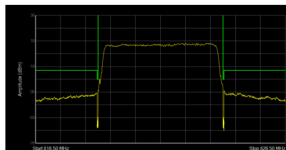
LTE Band 26 QPSK 5MHz CH-High 100%RB
