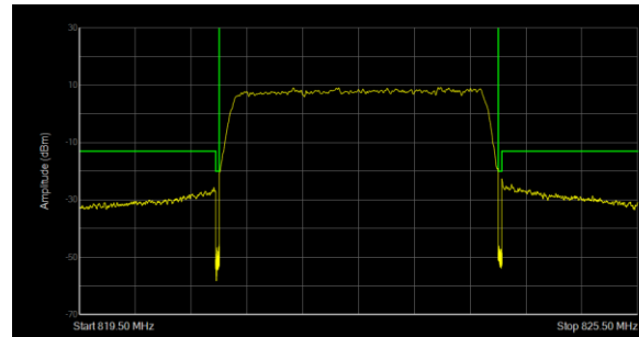
LTE Band 26 QPSK 3MHz CH-High 100%RB
