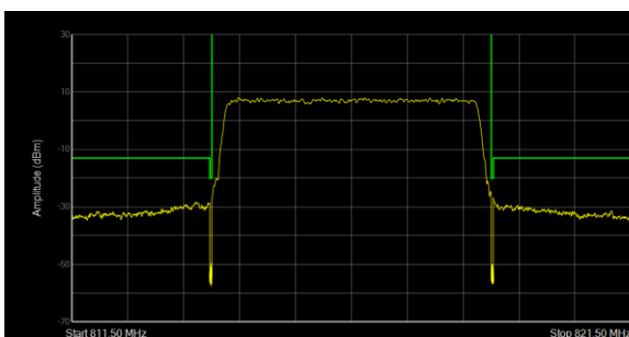
LTE Band 26 QPSK 5MHz CH-Low 100%RB
