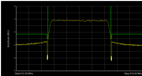
LTE Band 26 QPSK 3MHz CH-Low 100%RB
