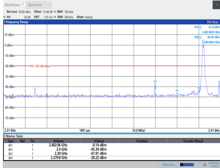
BLE_1M_Ant1_Low_2402
