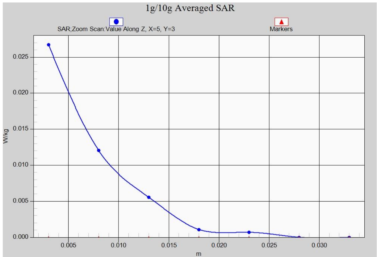
Fig. 13-1 Z-Scan at power reference point (LTE Band38)
