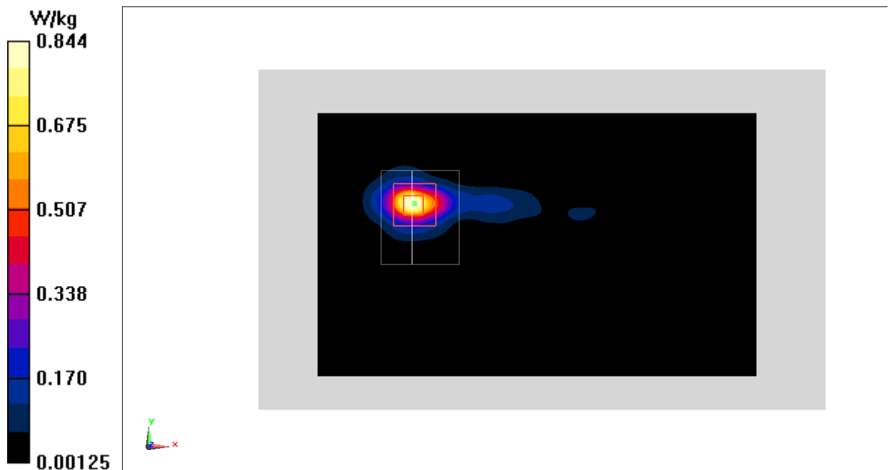
Fig.16 2450 MHz
