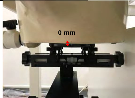
Fig.15 EUT Front side to flat phantom
