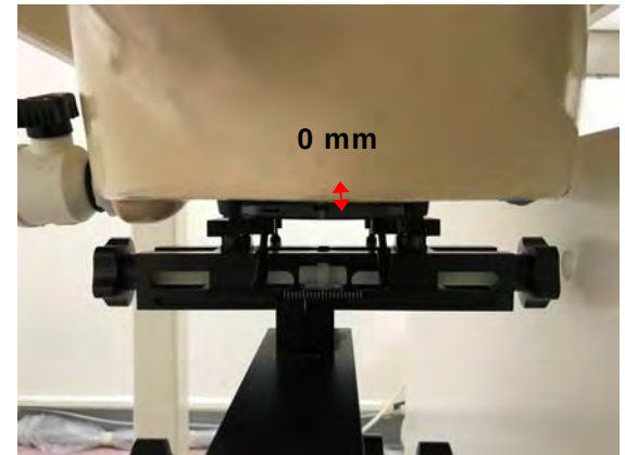
Fig.16 EUT Back side to flat phantom
