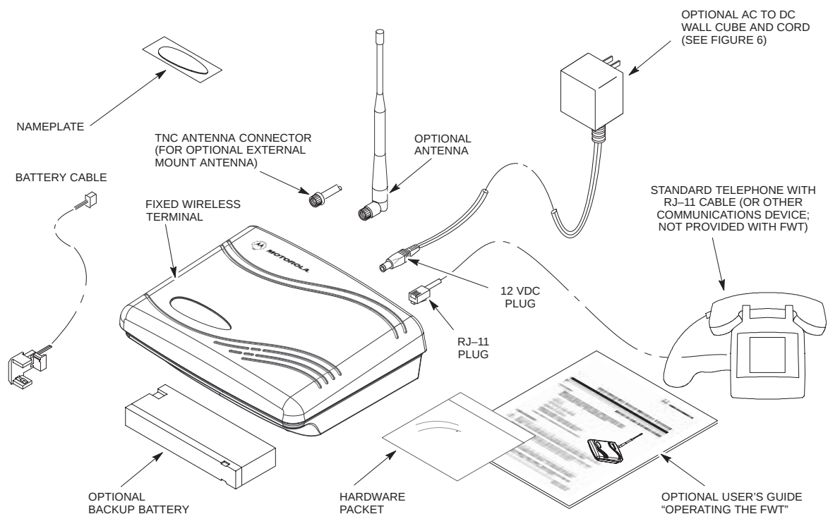
Figure 5: FWT components
