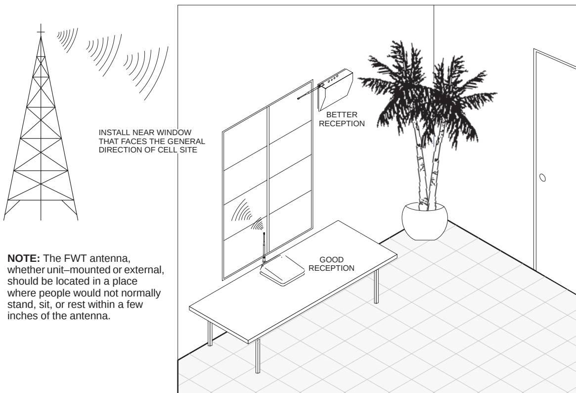
Figure 3: Preferred FWT locations without external antenna
