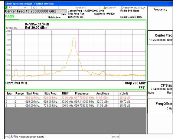
n71 5M DFT-s-OFDM QPSK Edge_1RB_Right High
