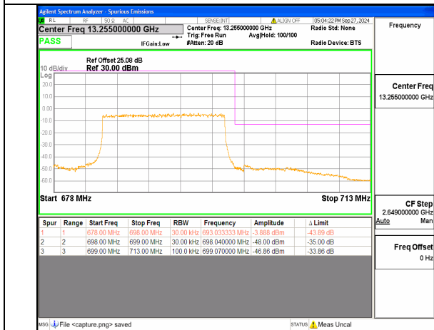
n71 15M DFT-s-OFDM BPSK Outer_Full High
