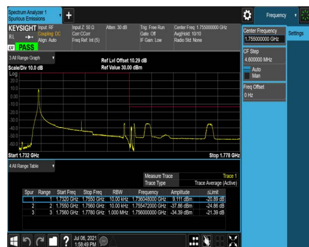
Band4-20MHz-16QAM-20300-100RB#0
