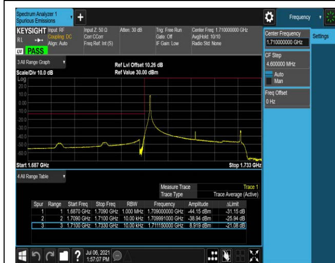
Band4-20MHz-16QAM-20050-100RB#0
