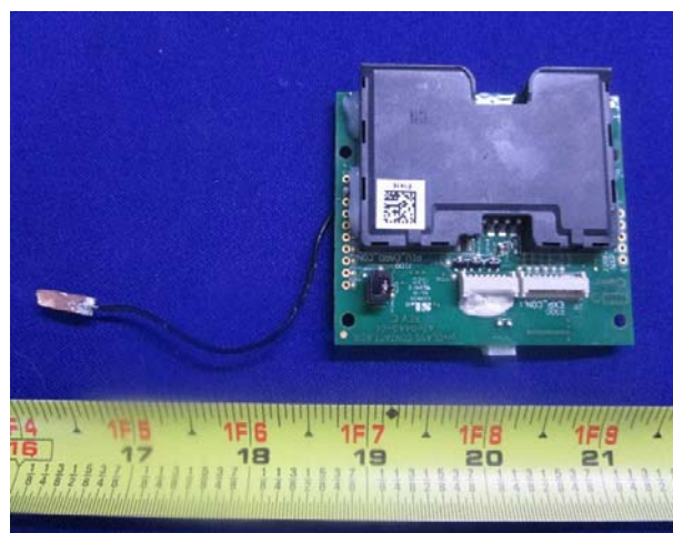
PCBA3 Bottom View
