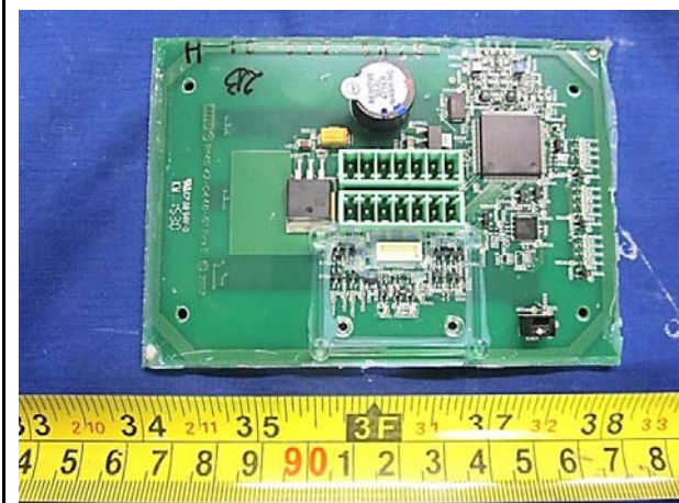
PCBA 1 Top View 1 without PCBA2
