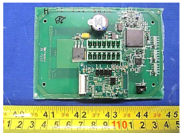
PCBA 1 Top View 2 with PCBA2
