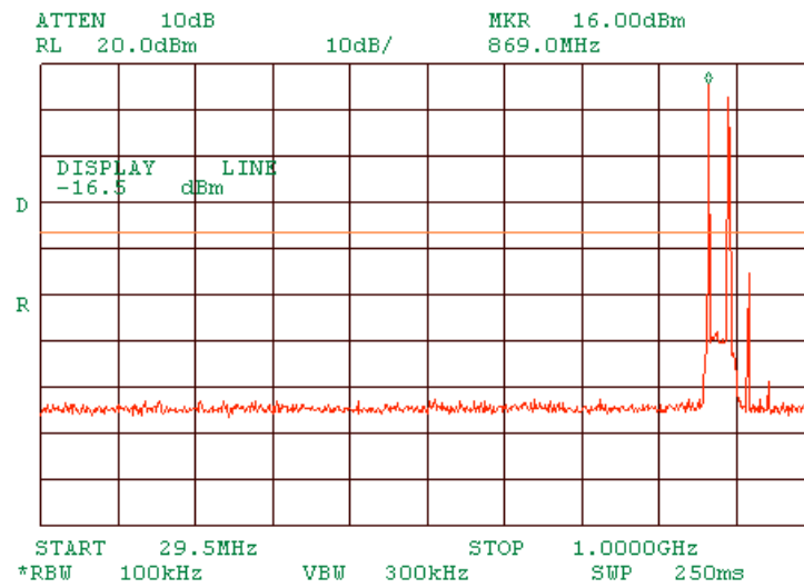
Plot 1.7.49 Spurious emission measurements in 30 - 1000 MHz range at high carrier frequency OFDM
