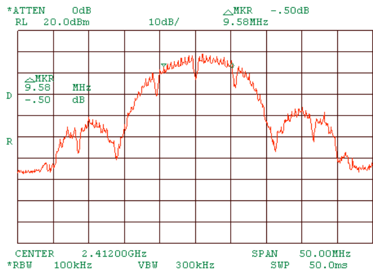
Plot 1.2.3 6 dB bandwidth test result at low frequency of MA 850 stands alone. At 11 Mbps DSSS.
