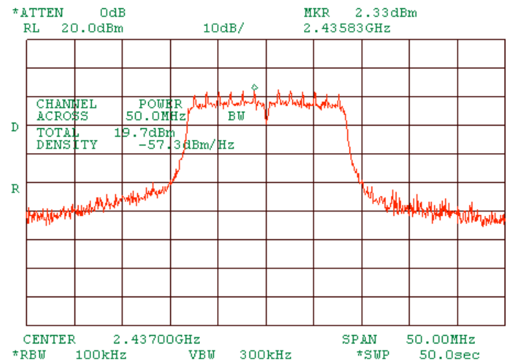
Plot 1.5.9 Peak output power at mid frequency of MA 850 and MA 1000 interconnected, port 1. At 9Mbps OFDM.
