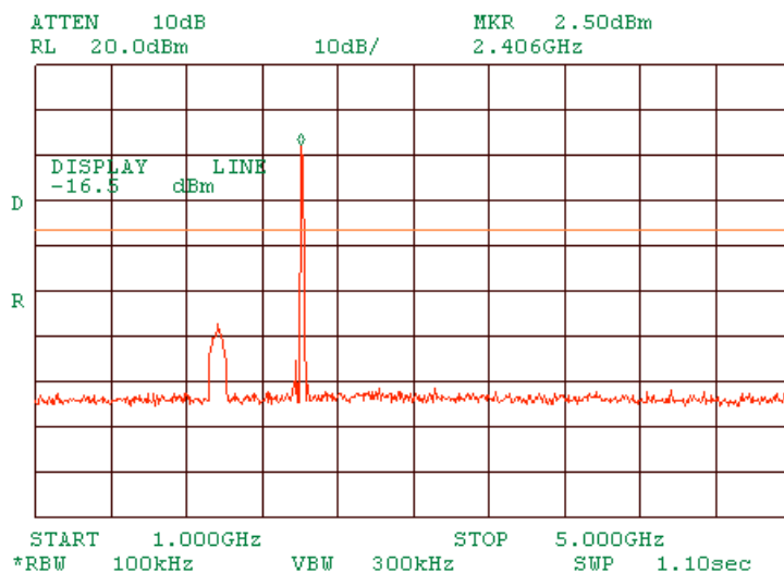
Plot 1.7.51 Spurious emission measurements in 1000 - 5000 MHz range at low carrier frequency OFDM
