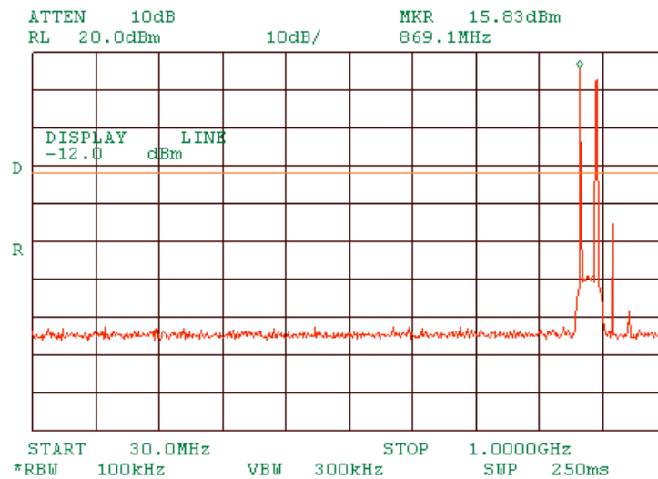
Plot 1.7.10 Spurious emission measurements in 30 - 1000 MHz range at low carrier frequency DSSS
