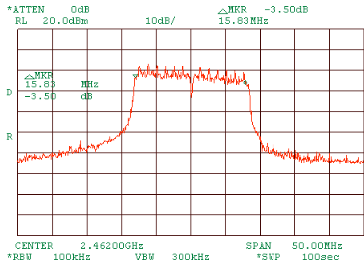
Plot 1.2.39 6 dB bandwidth test result at high frequency of MA 850 stands alone. At 54 Mbps OFDM.
