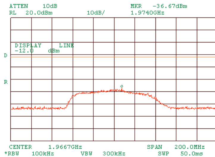
Plot 1.7.21 Zoom into spurious at high carrier frequency DSSS
