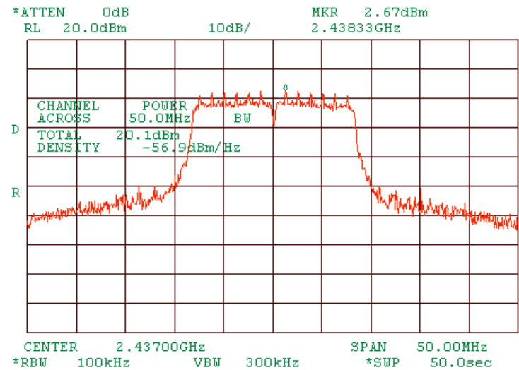
Plot 1.5.8 Peak output power at mid frequency of MA 850 and MA 1000 interconnected, port 1. At 6Mbps OFDM.
