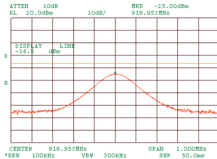
Plot 1.7.50 Zoom into spurious at mid carrier frequency OFDM
