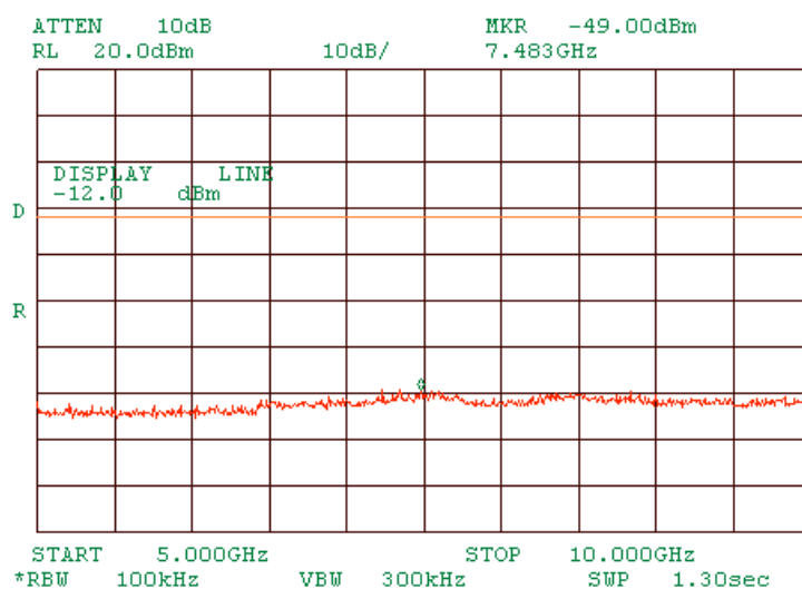
Plot 1.7.22 Spurious emission measurements in 5000 - 10000 MHz range at low carrier frequency DSSS
