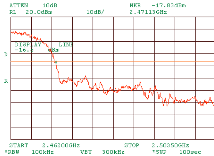
Plot 1.7.32 Band edge measurements at high carrier frequency DSSS
