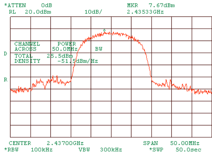
Plot 1.5.24 Peak output power at mid frequency of MA 850 and MA 1000 interconnected, port 3. At 5.5Mbps DSSS.
