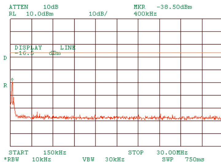
Plot 1.7.41 Spurious emission measurements in 0.15 - 30 MHz range at mid carrier frequency OFDM
