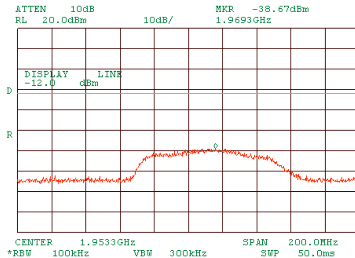
Plot 1.7.17 Zoom into spurious at mid carrier frequency DSSS
