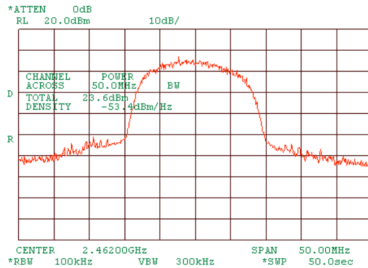
Plot 1.4.21 Peak output power at high frequency of MA 850 and MA 1000 interconnected, port 4. At 5.5Mbps DSSS.
