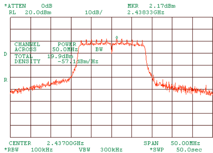
Plot 1.6.5 Peak output power at mid frequency of MA 850, port 1. At 6Mbps OFDM.
