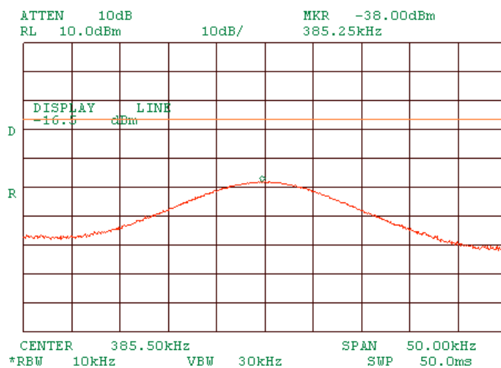
Plot 1.7.42 Zoom into spurious at mid carrier frequency OFDM
