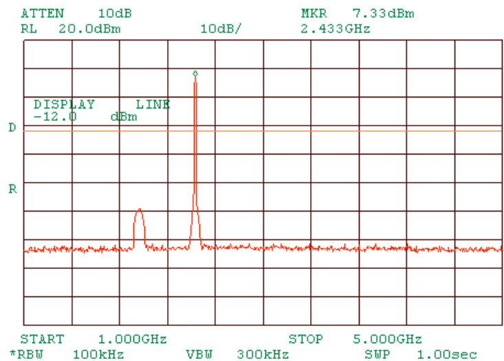
Plot 1.7.18 Spurious emission measurements in 1000 - 5000 MHz range at mid carrier frequency DSSS
