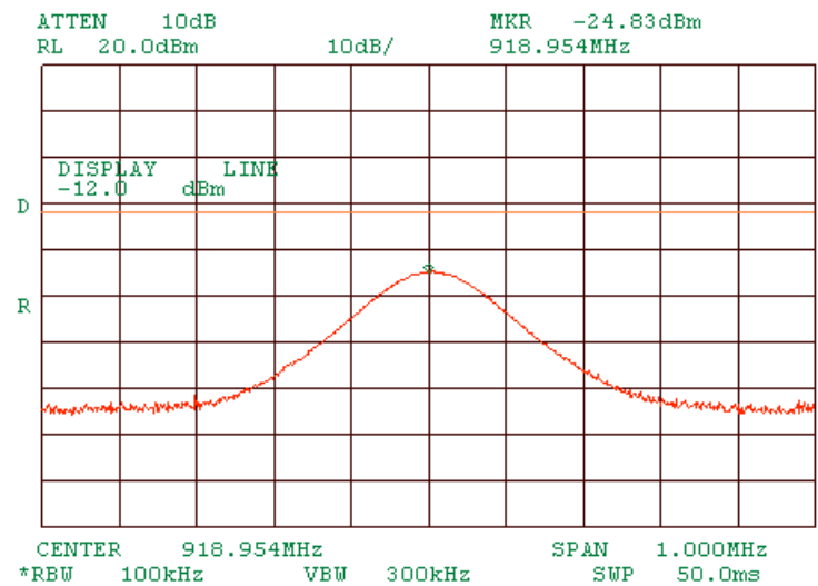
Plot 1.7.13 Zoom into spurious at mid carrier frequency DSSS
