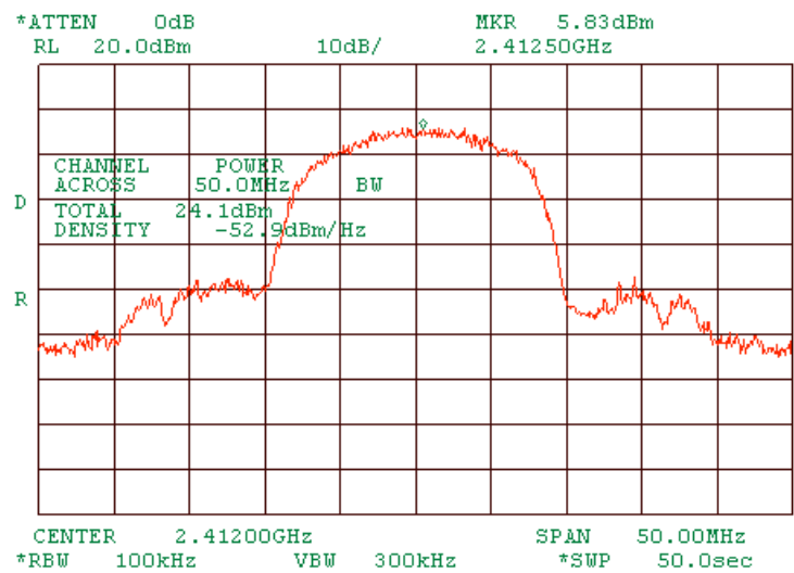
Plot 1.5.29 Peak output power at low frequency of MA 850 and MA 1000 interconnected, port 4. At 5.5Mbps DSSS.
