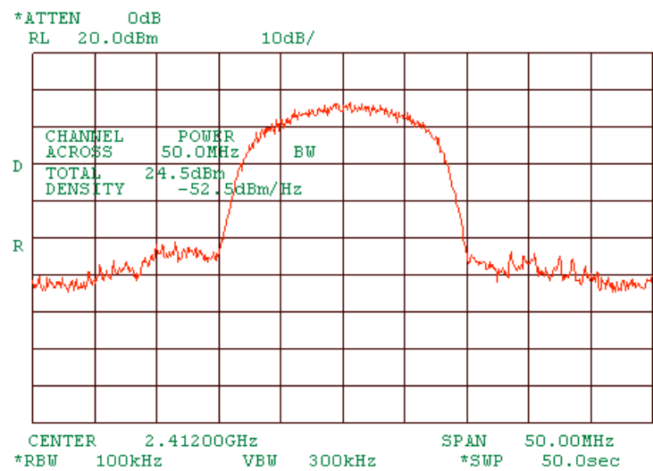
Plot 1.4.19 Peak output power at low frequency of MA 850 and MA 1000 interconnected, port 4. At 5.5Mbps DSSS.
