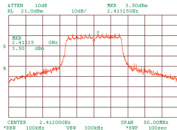
Plot 1.7.33 The highest emission level within the assigned band at low carrier frequency OFDM
