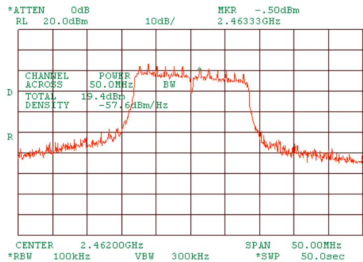
Plot 1.5.16 Peak output power at high frequency of MA 850 and MA 1000 interconnected, port 1. At 6 Mbps OFDM.
