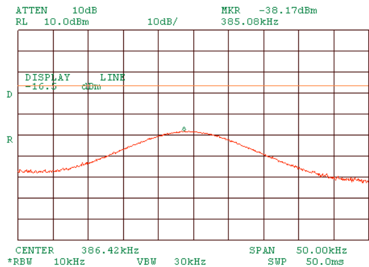
Plot 1.7.40 Zoom into spurious at low carrier frequency OFDM
