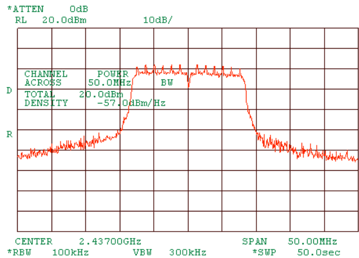
Plot 1.4.5 Peak output power at mid frequency of MA 850 and MA 1000 interconnected, port 1. At 6Mbps OFDM.
