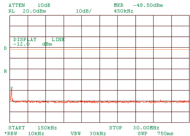
Plot 1.7.8 Spurious emission measurements in 0.15 - 30 MHz range at mid carrier frequency DSSS
