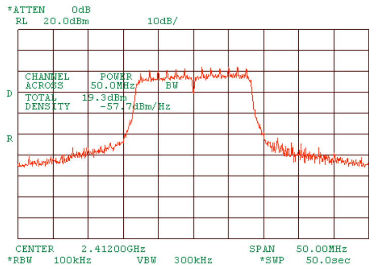
Plot 1.6.16 Peak output power at low frequency of MA 850, port 3. At 6Mbps OFDM.
