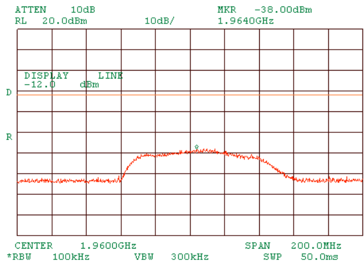
Plot 1.7.19 Zoom into spurious at mid carrier frequency DSSS
