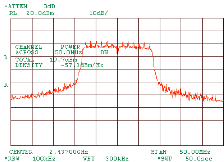
Plot 1.6.17 Peak output power at mid frequency of MA 850, port 3. At 6Mbps OFDM.
