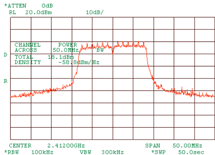
Plot 1.6.22 Peak output power at low frequency of MA 850, port 4. At 6Mbps OFDM.
