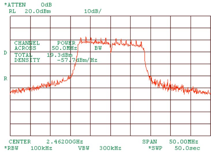
Plot 1.4.6 Peak output power at high frequency of MA 850 and MA 1000 interconnected, port 1. At 6 Mbps OFDM.
