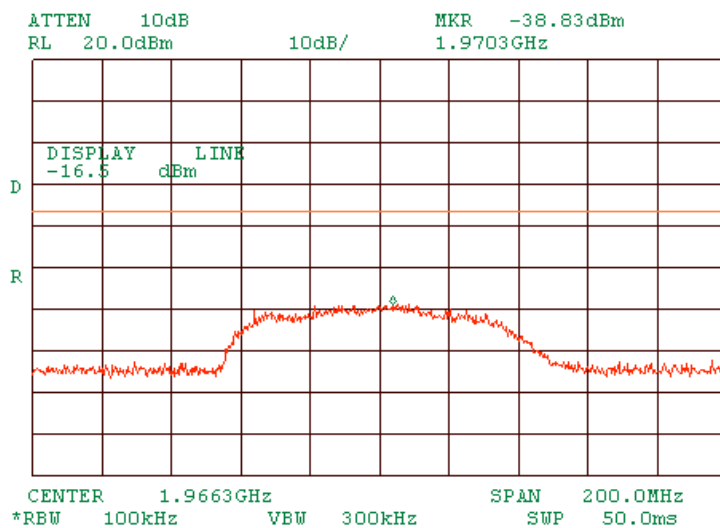
Plot 1.7.52 Zoom into spurious at mid carrier frequency OFDM
