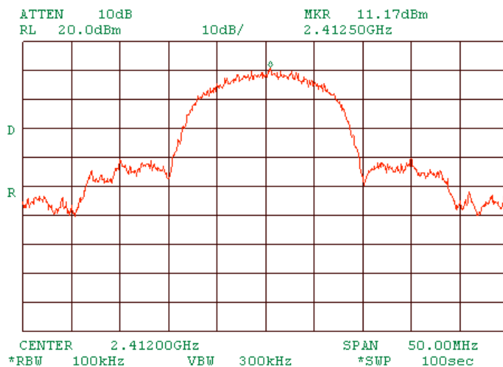
Plot 1.7.1 The highest emission level within the assigned band at low carrier frequency DSSS
