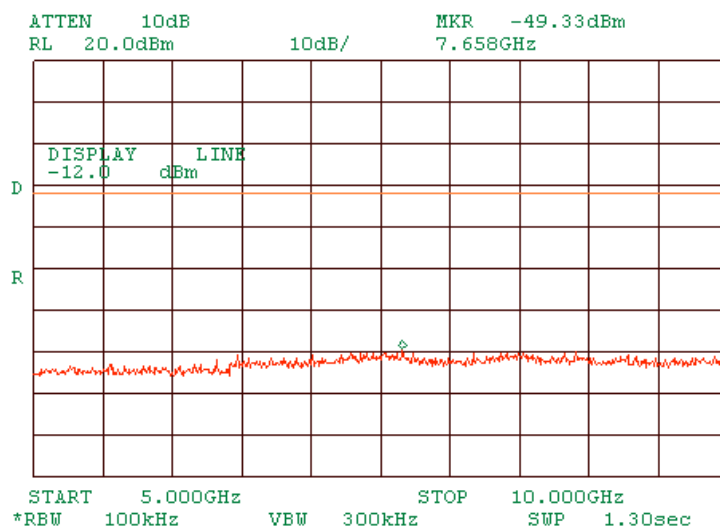
Plot 1.7.23 Spurious emission measurements in 5000 - 10000 MHz range at mid carrier frequency DSSS
