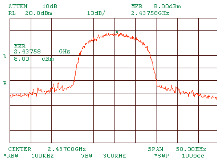
Plot 1.7.2 The highest emission level within the assigned band at mid carrier frequency DSSS
