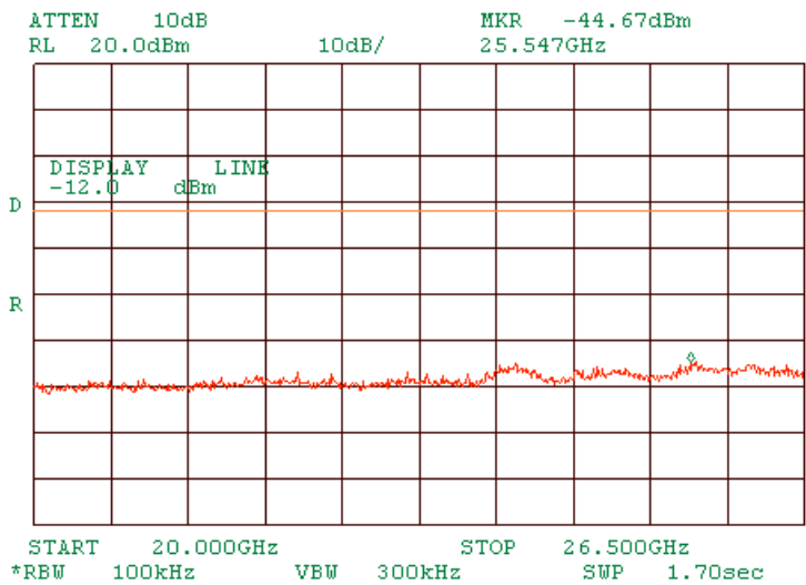
Plot 1.7.29 Spurious emission measurements in 20000 - 26500 MHz range at mid carrier frequency DSSS
