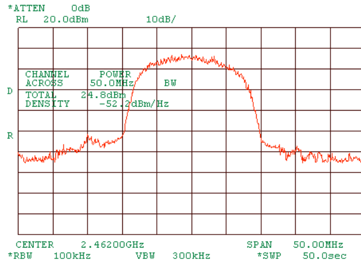
Plot 1.4.15 Peak output power at high frequency of MA 850 and MA 1000 interconnected, port 3. At 5.5Mbps DSSS.
