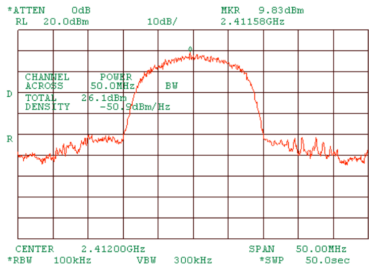
Plot 1.5.17 Peak output power at low frequency of MA 850 and MA 1000 interconnected, port 2. At 5.5Mbps DSSS.
