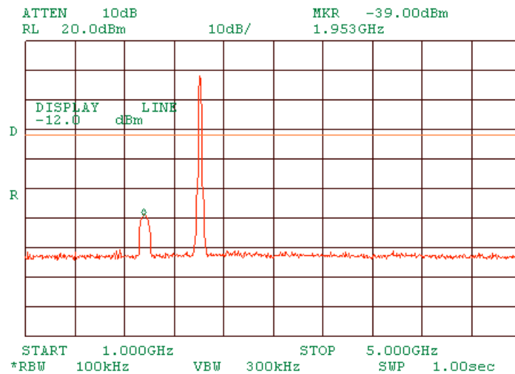
Plot 1.7.16 Spurious emission measurements in 1000 - 5000 MHz range at low carrier frequency DSSS
