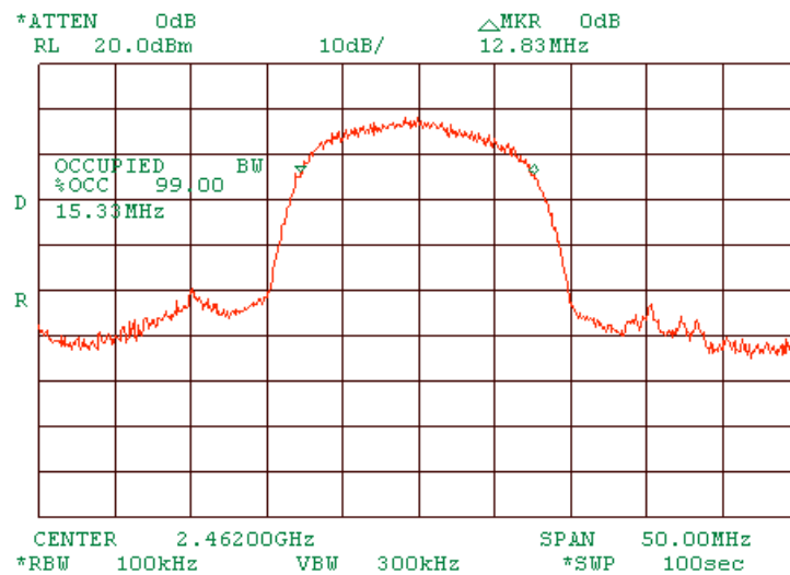
Plot 1.3.12 99% power bandwidth test result at high frequency with MA 850 and MA 1000 interconnected. At 11 Mbps DSSS.
