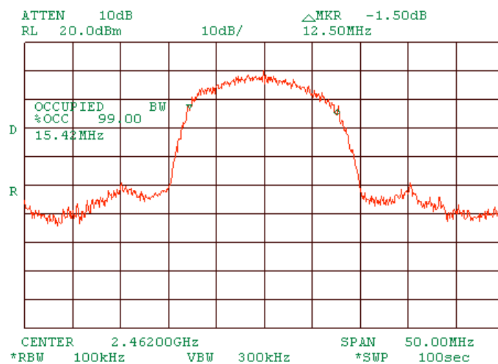
Plot 1.1.12 99% power bandwidth test result at high frequency with MA 850 and MA 1000 interconnected. At 11 Mbps DSSS.
