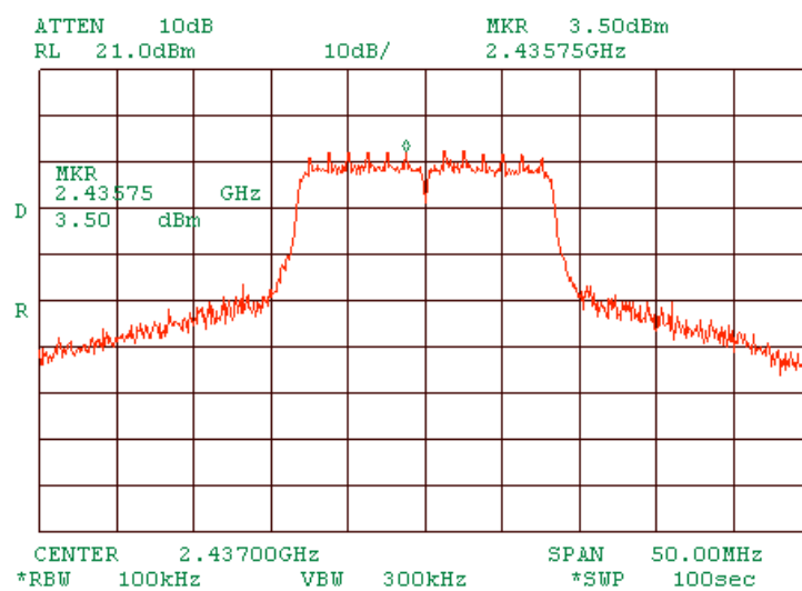
Plot 1.7.34 The highest emission level within the assigned band at mid carrier frequency OFDM
