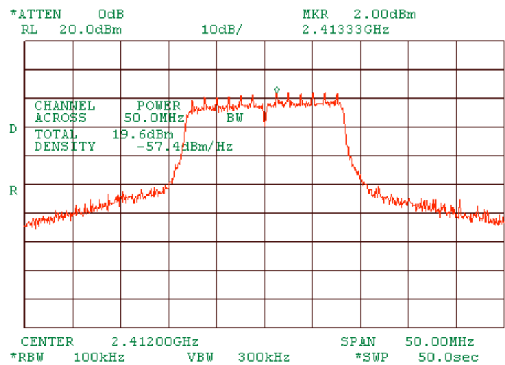
Plot 1.5.7 Peak output power at low frequency of MA 850 and MA 1000 interconnected, port 1. At 6 Mbps OFDM.
