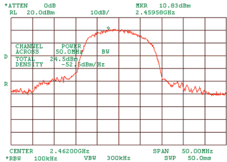
Plot 1.5.6 Peak output power at high frequency of MA 850 and MA 1000 interconnected, port 1. At 5.5Mbps DSSS.
