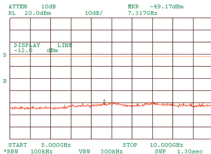
Plot 1.7.24 Spurious emission measurements in 5000 - 10000 MHz range at high carrier frequency DSSS
