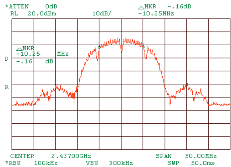
Plot 1.2.9 6 dB bandwidth test result at mid frequency of MA 850 stands alone. At 5.5 Mbps DSSS.
