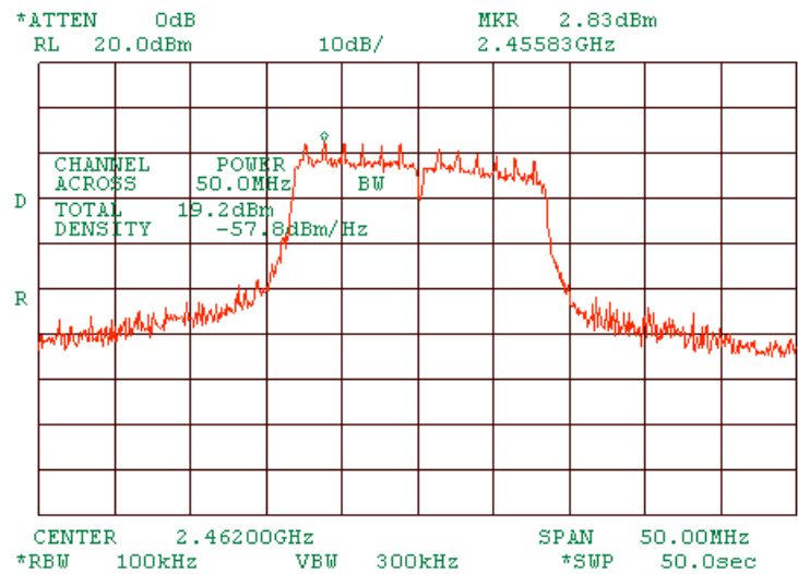
Plot 1.6.6 Peak output power at high frequency of MA 850, port 1. At 6 Mbps OFDM.
