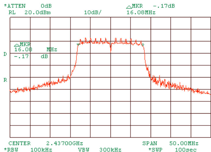
Plot 1.2.23 6 dB bandwidth test result at mid frequency of MA 850 stands alone. At 9 Mbps OFDM.
