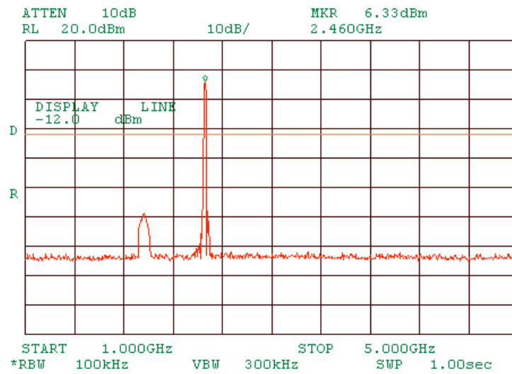
Plot 1.7.20 Spurious emission measurements in 1000 - 5000 MHz range at high carrier frequency DSSS
