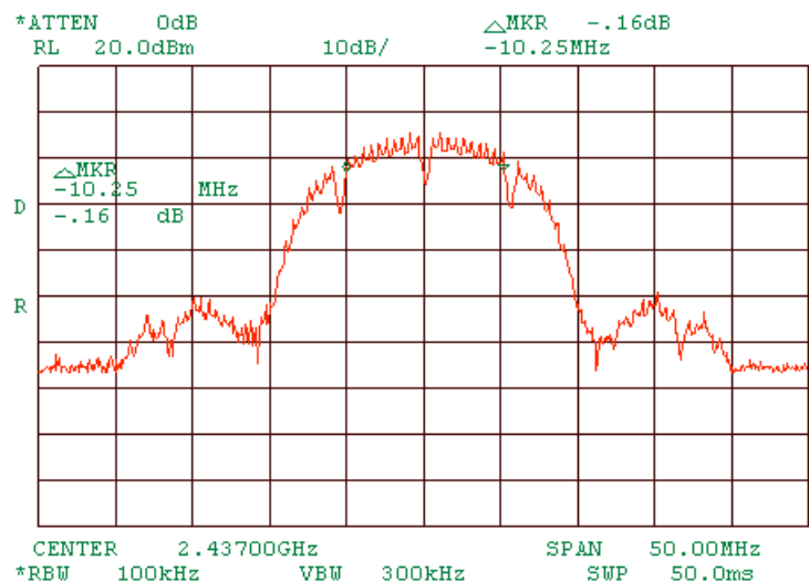
Plot 1.2.11 6 dB bandwidth test result at mid frequency of MA 850 stands alone. At 11 Mbps DSSS.
