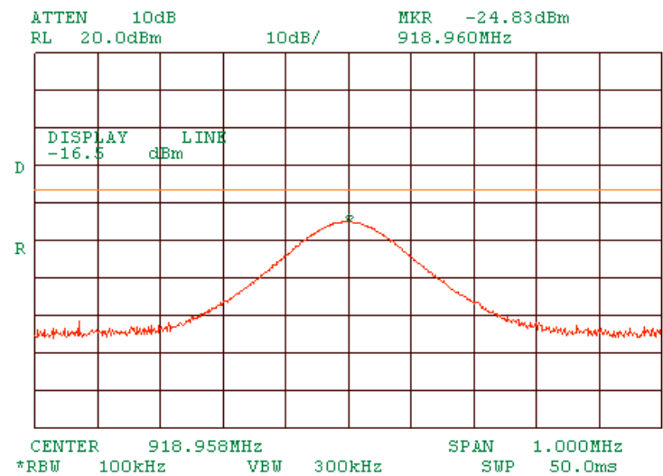
Plot 1.7.48 Zoom into spurious at mid carrier frequency OFDM
