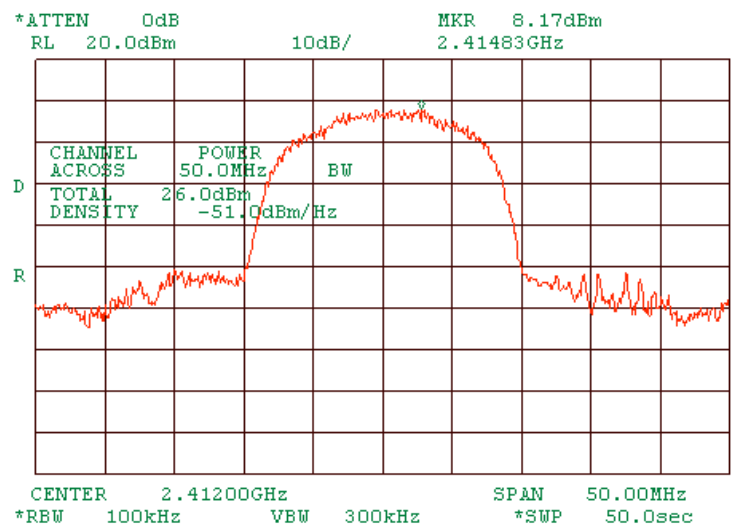
Plot 1.6.7 Peak output power at low frequency of MA 850, port 2. At 5.5Mbps DSSS.
