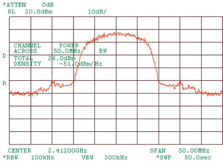
Plot 1.4.13 Peak output power at low frequency of MA 850 and MA 1000 interconnected, port 3. At 5.5Mbps DSSS.
