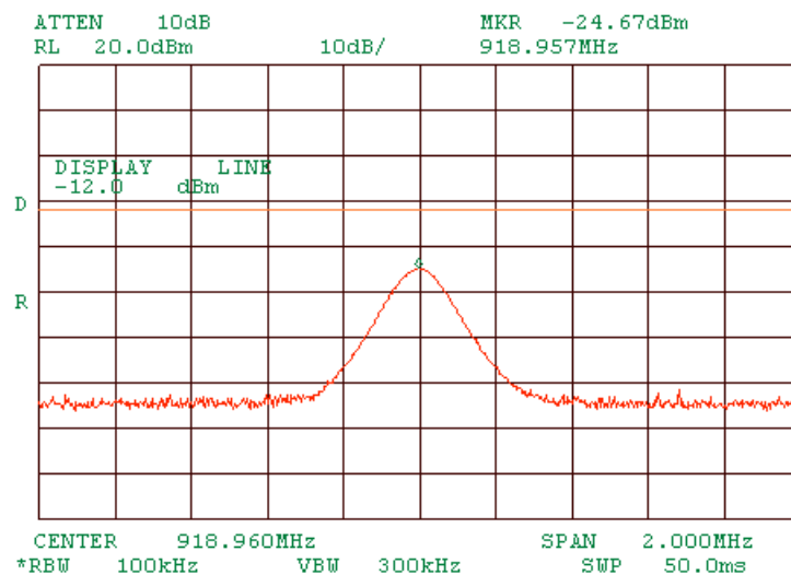
Plot 1.7.11 Zoom into spurious at low carrier frequency DSSS
