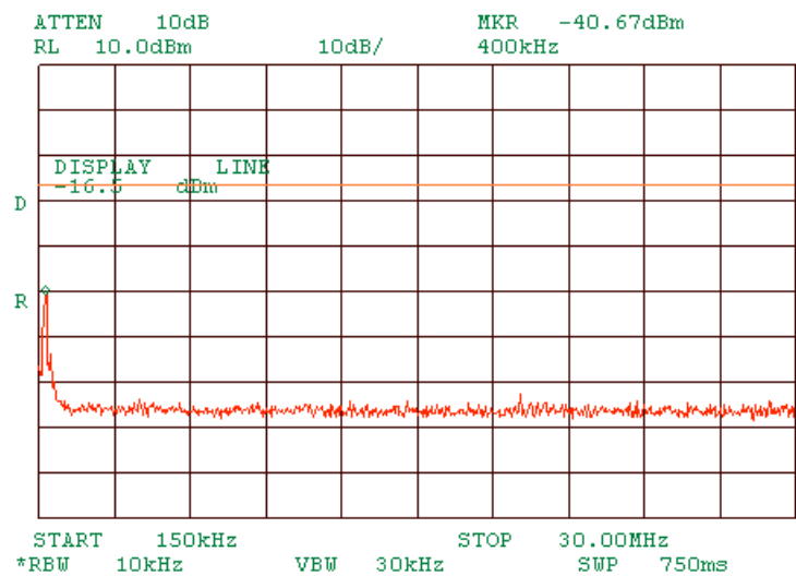
Plot 1.7.39 Spurious emission measurements in 0.15 - 30 MHz range at low carrier frequency OFDM
