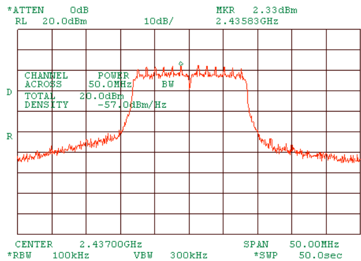
Plot 1.5.11 Peak output power at mid frequency of MA 850 and MA 1000 interconnected, port 1. At 18Mbps OFDM.
