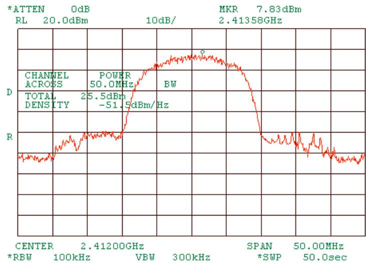
Plot 1.5.23 Peak output power at low frequency of MA 850 and MA 1000 interconnected, port 3. At 5.5Mbps DSSS.
