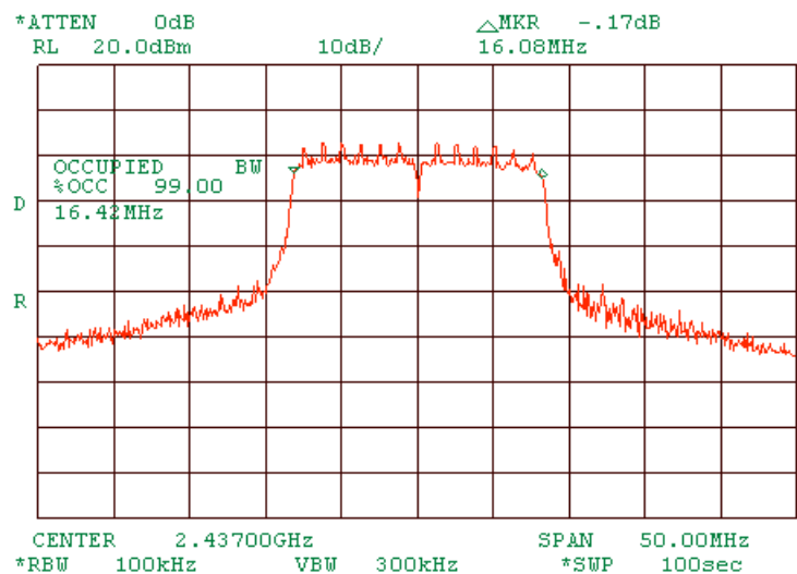
Plot 1.2.24 99% power bandwidth test result at mid frequency of MA 850 stands alone. At 9 Mbps OFDM.
