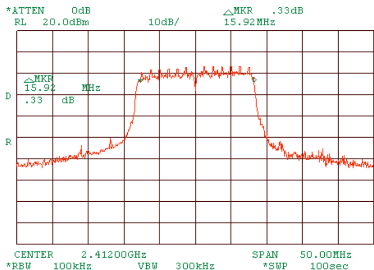
Plot 1.2.19 6 dB bandwidth test result at low frequency of MA 850 stands alone. At 54 Mbps OFDM.
