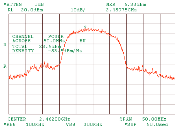
Plot 1.5.31 Peak output power at high frequency of MA 850 and MA 1000 interconnected, port 4. At 5.5Mbps DSSS.
