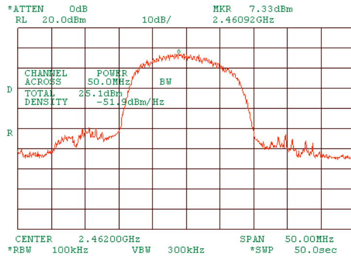
Plot 1.5.25 Peak output power at high frequency of MA 850 and MA 1000 interconnected, port 3. At 5.5Mbps DSSS.
