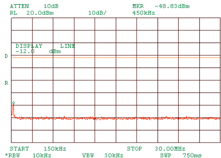
Plot 1.7.7 Spurious emission measurements in 0.15 - 30 MHz range at low carrier frequency DSSS
