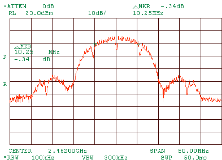
Plot 1.2.15 6 dB bandwidth test result at high frequency of MA 850 stands alone. At 11 Mbps DSSS.
