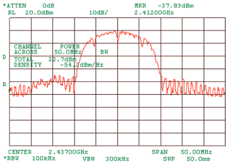
Plot 1.5.3 Peak output power at mid frequency of MA 850 and MA 1000 interconnected, port 1. At 2Mbps DSSS.
