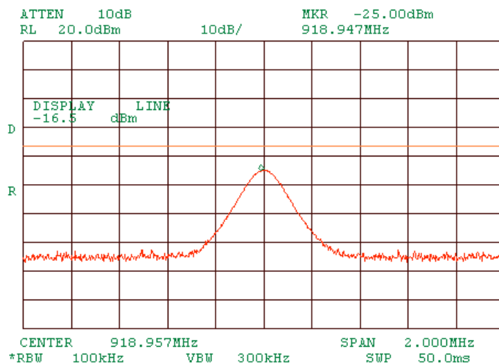
Plot 1.7.46 Zoom into spurious at low carrier frequency OFDM
