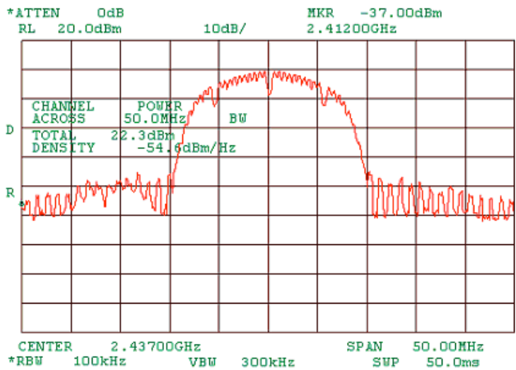
Plot 1.5.2 Peak output power at mid frequency of MA 850 and MA 1000 interconnected, port 1. At 1Mbps DSSS.
