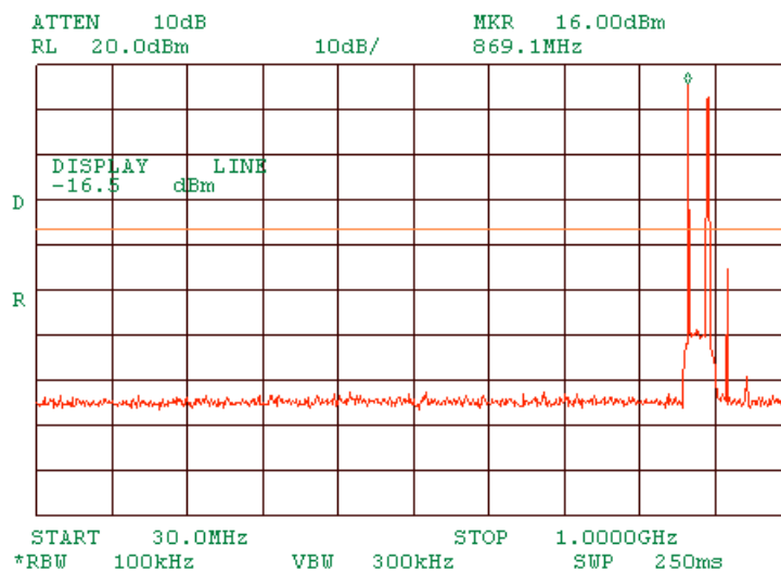
Plot 1.7.45 Spurious emission measurements in 30 - 1000 MHz range at low carrier frequency OFDM
