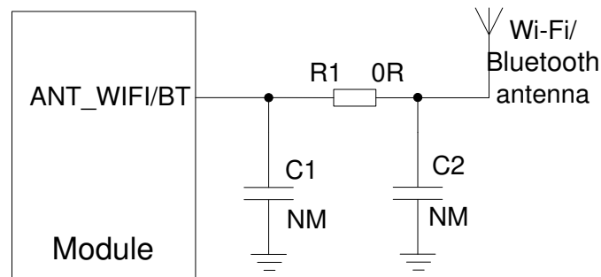
Figure 31: Reference Circuit Design for Wi-Fi/Bluetooth Antenna
