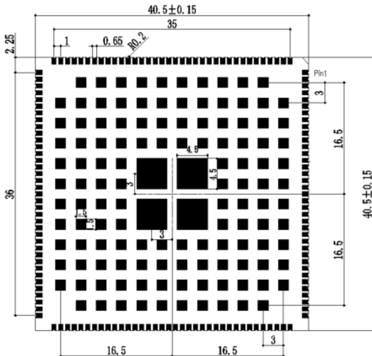
Figure 42: Bottom Dimension (Bottom View)
