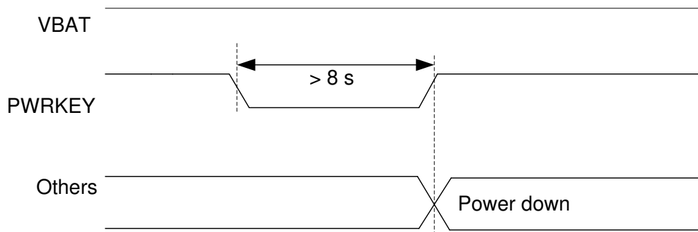
Figure 9: Timing of Turning Off the Module
