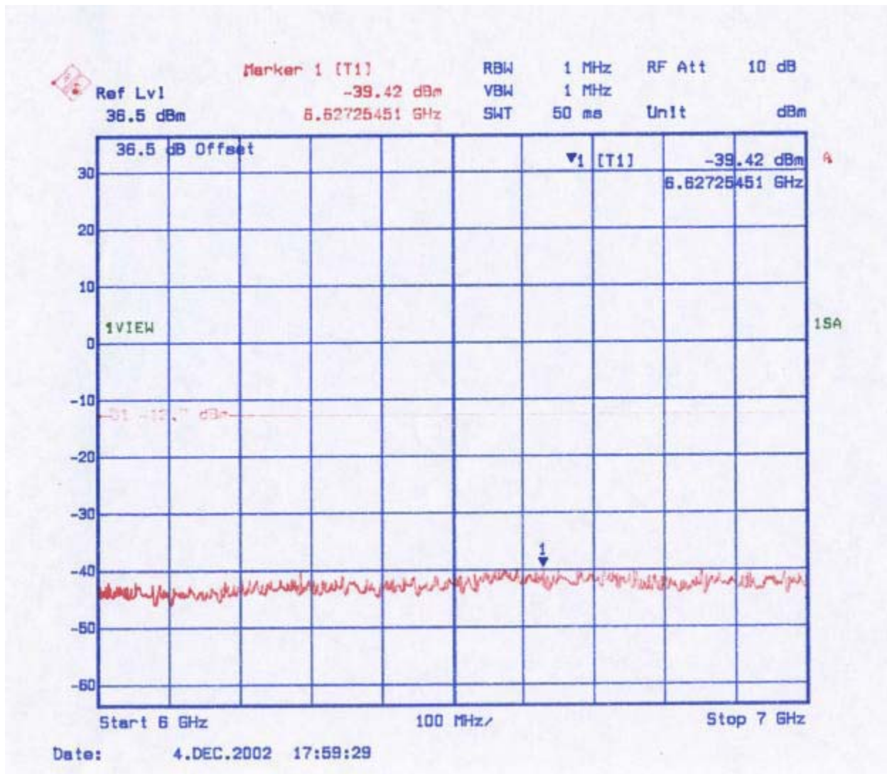
Figure 24: Conducted Spurious Emissions - 1 Carrier Channel 4 (6 GHz – 7 GHz)
