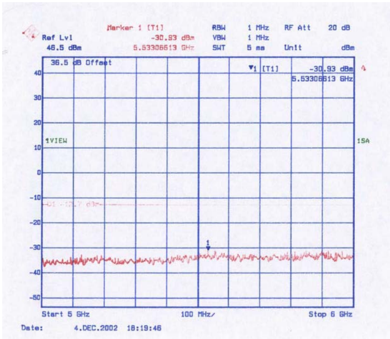
Figure 23: Conducted Spurious Emissions - 1 Carrier Channel 4 (5 GHz – 6 GHz)
