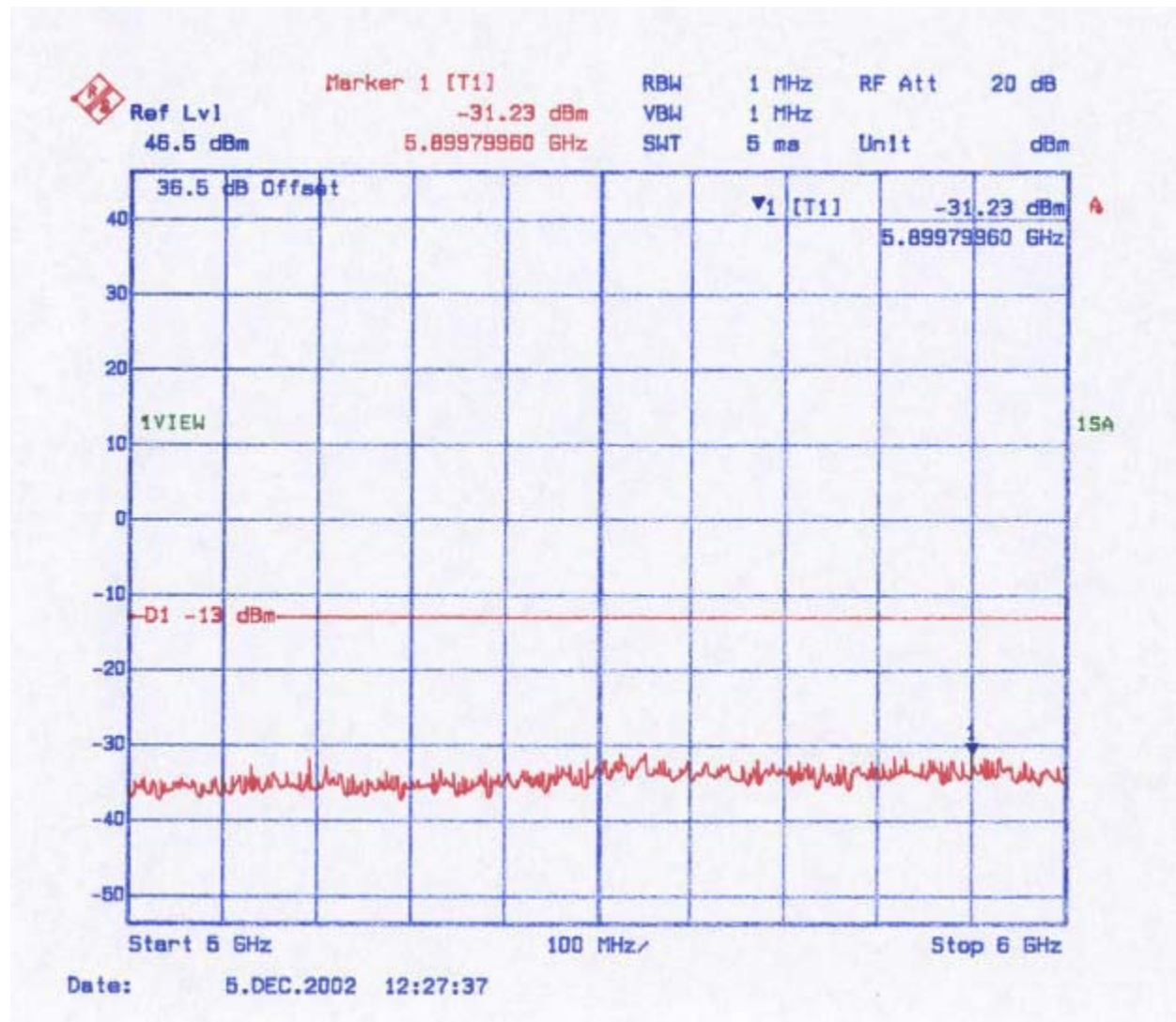
Figure 36: Conducted Spurious Emissions - 3 Carrier Channels 4, 45, 86 (5 GHz–6 GHz)
