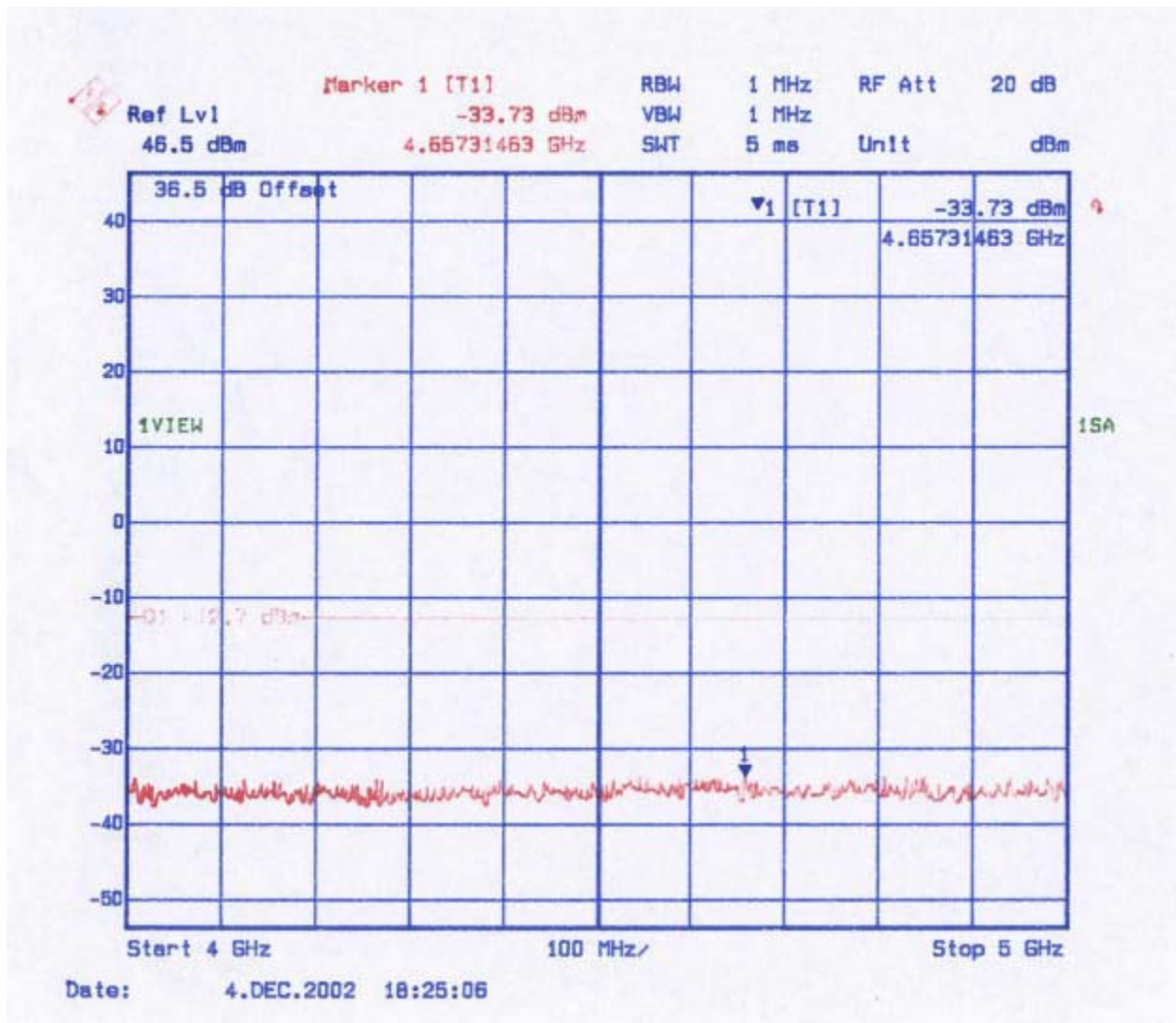
Figure 22: Conducted Spurious Emissions - 1 Carrier Channel 4 (4 GHz – 5 GHz)
