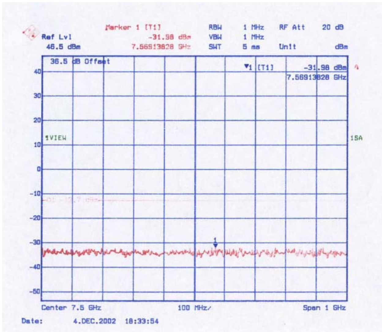
Figure 25: Conducted Spurious Emissions - 1 Carrier Channel 4 (7 GHz – 8 GHz)
