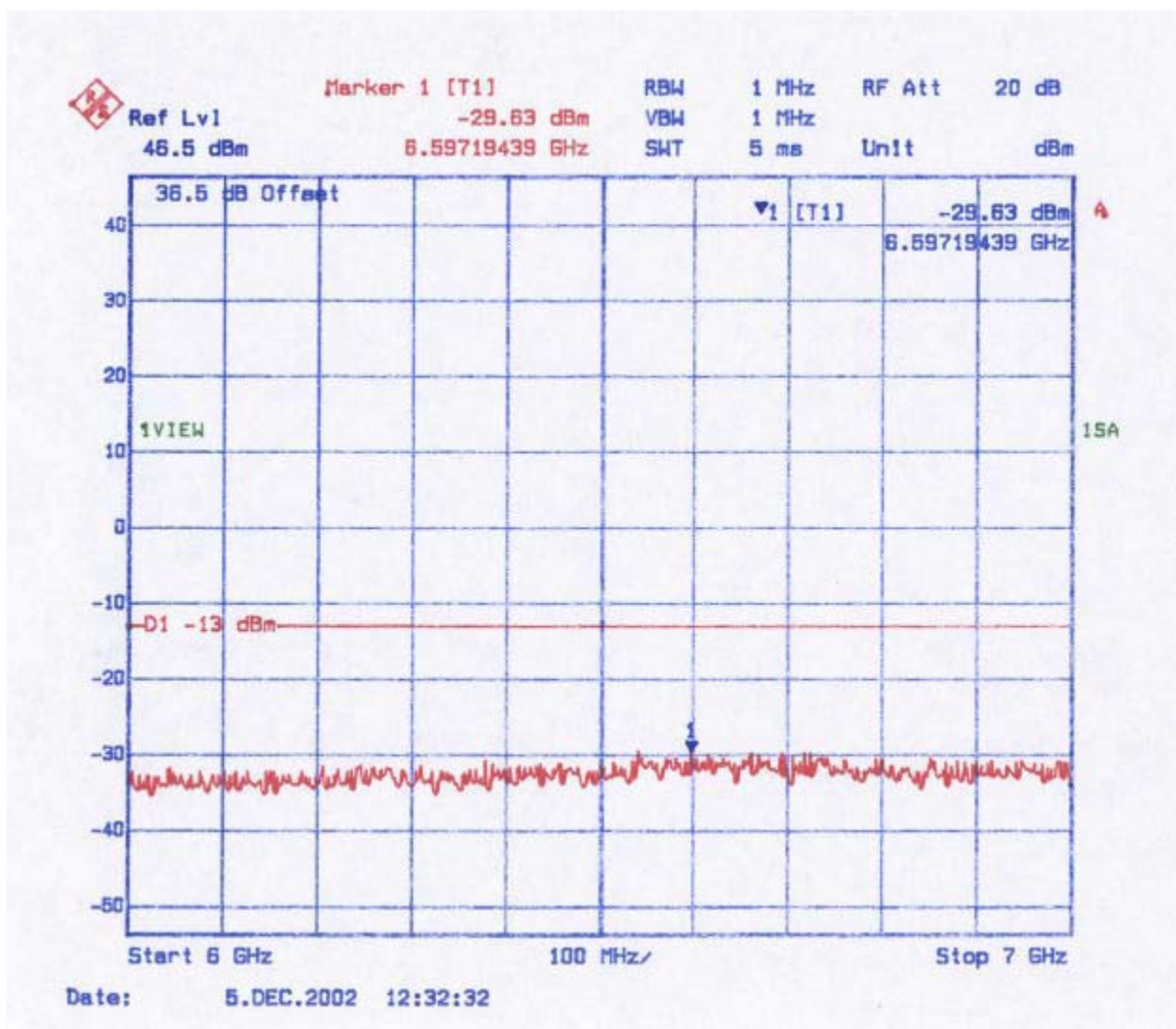
Figure 37: Conducted Spurious Emissions - 3 Carrier Channels 4, 45, 86 (6 GHz–7 GHz)
