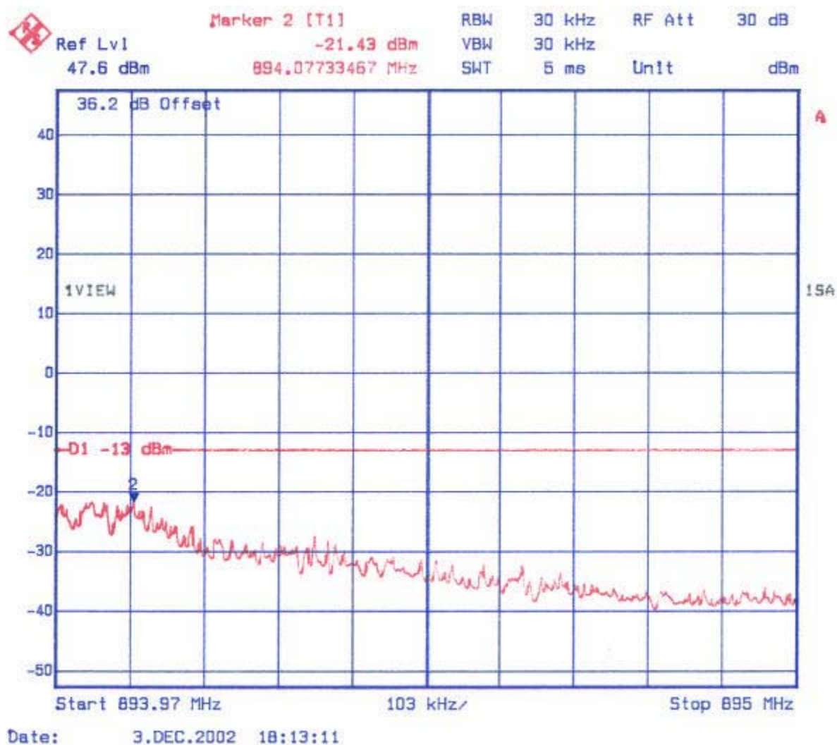
Figure 16: Spurious Emissions - 1 Carrier(Upper Band edge, adjacent 1 MHz)
