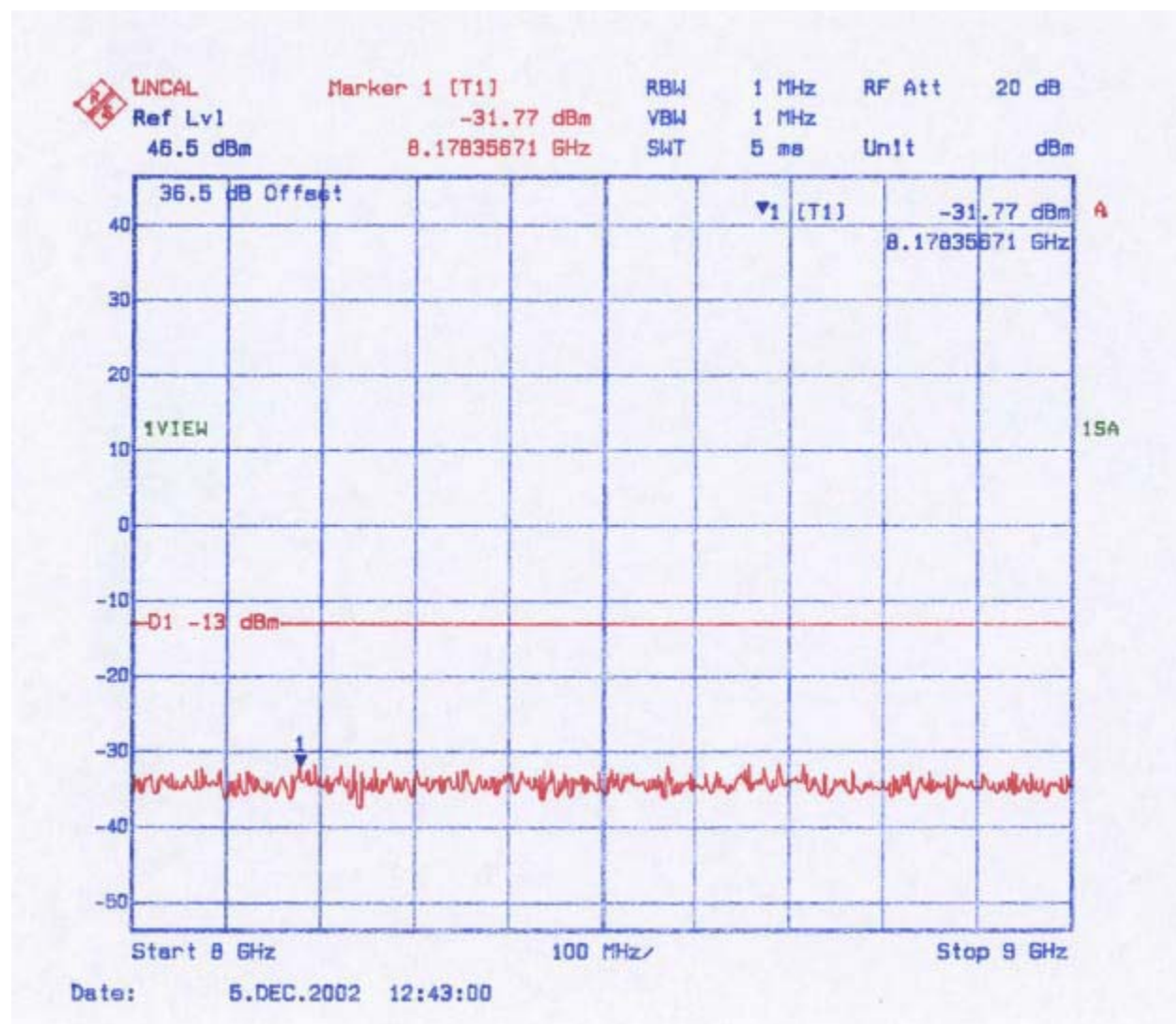
Figure 39: Conducted Spurious Emissions - 3 Carrier Channels 4, 45, 86 (8 GHz-9 GHz)
