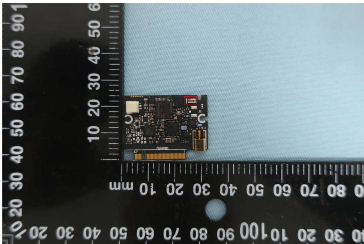
Bluetooth BR/EDR / Bluetooth LE: Chip Antenna (Ant1)
