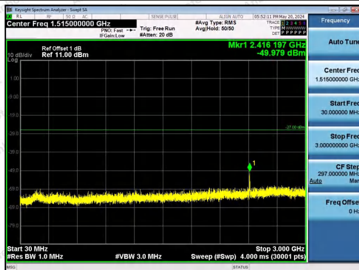
11AX80SISO-Ant1-7025-484Tone-RU66-30~3000-PASS
