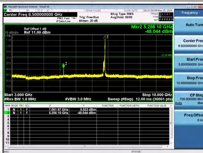
11AX80SISO-Ant1-7025-52Tone-RU52-3000~10000-PASS
