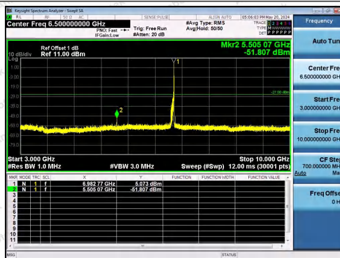
11AX80SISO-Ant1-6945-26Tone-RU36-3000~10000-PASS
