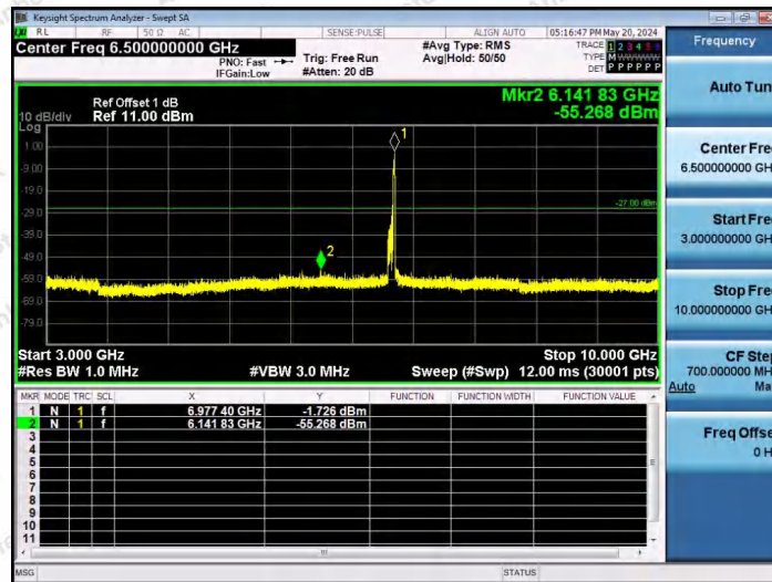
11AX80SISO-Ant1-6945-106Tone-RU60-3000~10000-PASS
