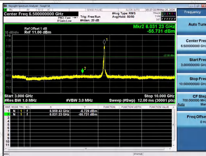
11AX80SISO-Ant1-6945-484Tone-RU66-3000~10000-PASS
