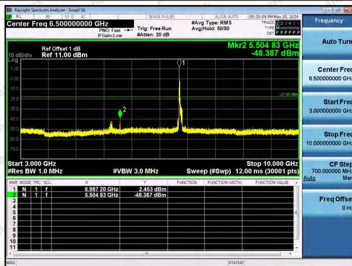
11AX80SISO-Ant1-7025-26Tone-RU0-3000~10000-PASS
