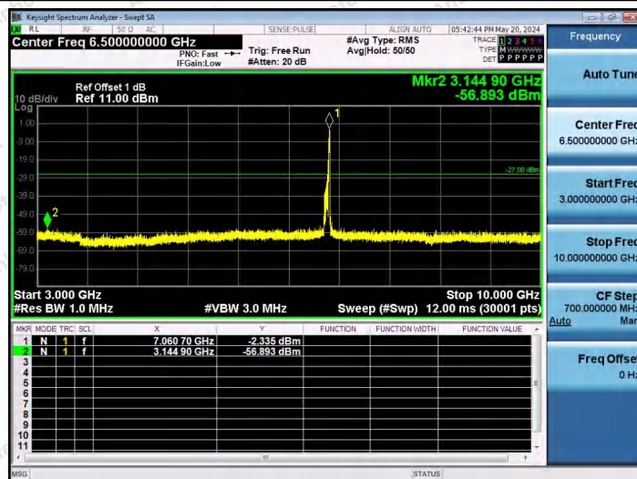
11AX80SISO-Ant1-7025-106Tone-RU60-3000~10000-PASS
