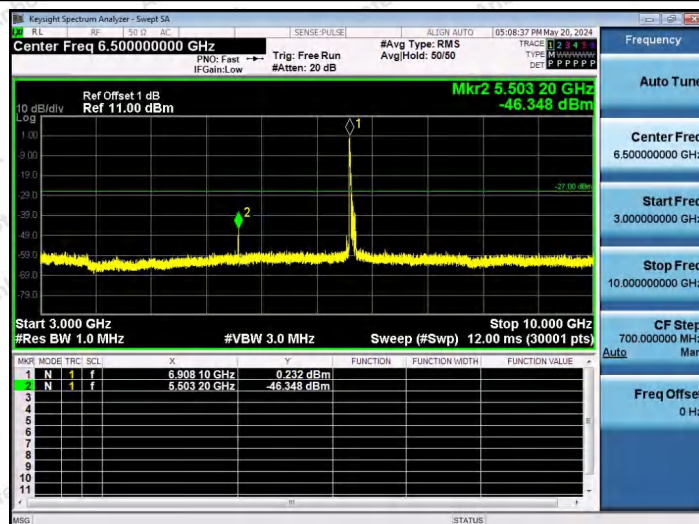
11AX80SISO-Ant1-6945-52Tone-RU37-3000~10000-PASS
