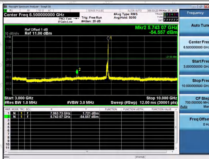
11AX80SISO-Ant1-7025-26Tone-RU36-3000~10000-PASS
