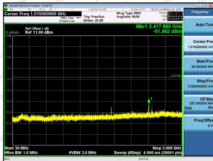
11AX80SISO-Ant1-7025-26Tone-RU36-30~3000-PASS
