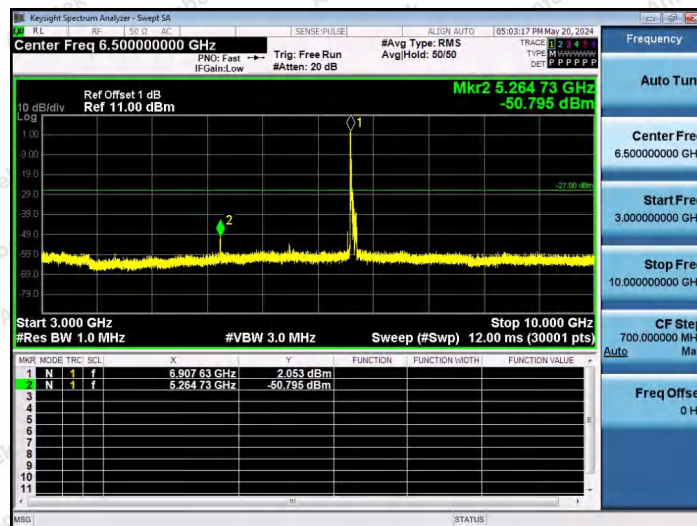
11AX80SISO-Ant1-6945-26Tone-RU0-3000~10000-PASS
