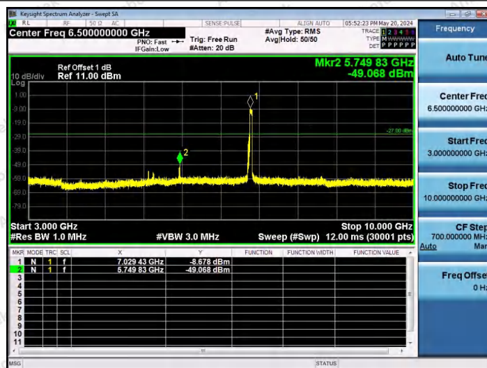
11AX80SISO-Ant1-7025-484Tone-RU66-3000~10000-PASS
