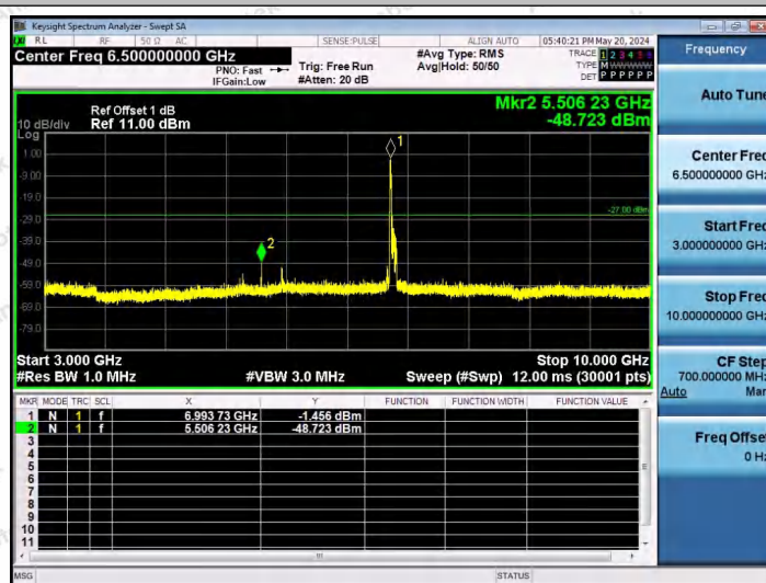
11AX80SISO-Ant1-7025-106Tone-RU53-3000~10000-PASS
