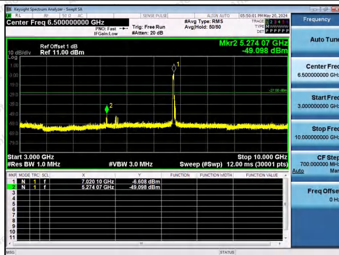
11AX80SISO-Ant1-7025-484Tone-RU65-3000~10000-PASS
