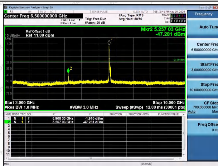
11AX80SISO-Ant1-6945-106Tone-RU53-3000~10000-PASS
