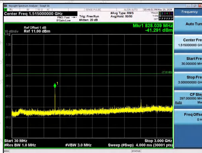
11AX80SISO-Ant1-7025-484Tone-RU65-30~3000-PASS
