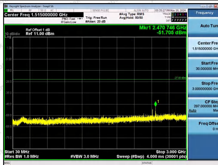
11AX80SISO-Ant1-7025-52Tone-RU37-30~3000-PASS
