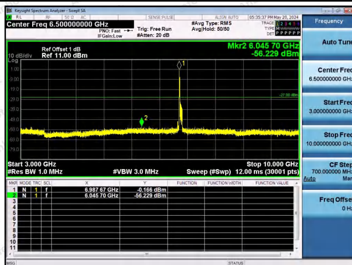
11AX80SISO-Ant1-7025-52Tone-RU37-3000~10000-PASS
