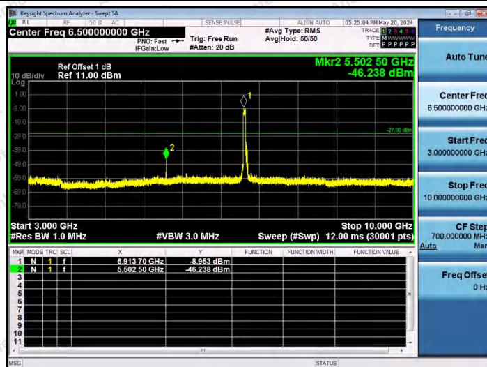
11AX80SISO-Ant1-6945-484Tone-RU65-3000~10000-PASS
