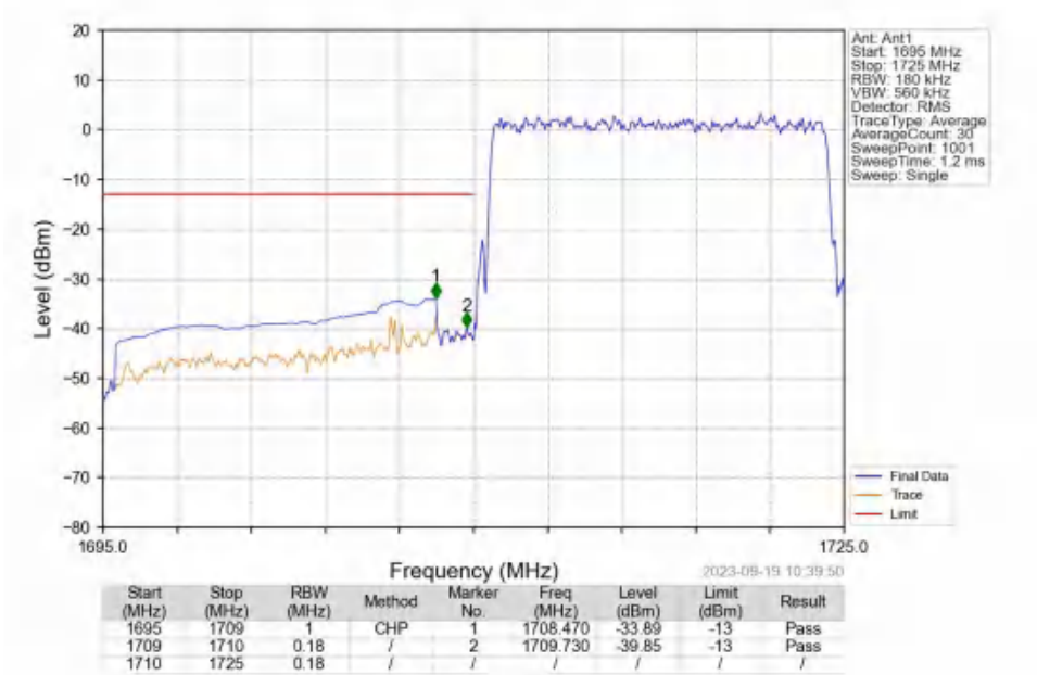
Band4_15MHz_QPSK_LCH_1717.5MHz_RB_75_0_NTNV
