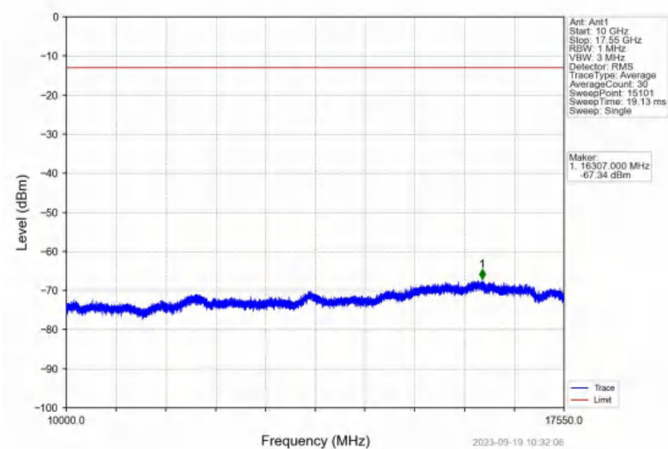
Band4_10MHz_16QAM_LCH_1715MHz_RB_50_0_NTNV
