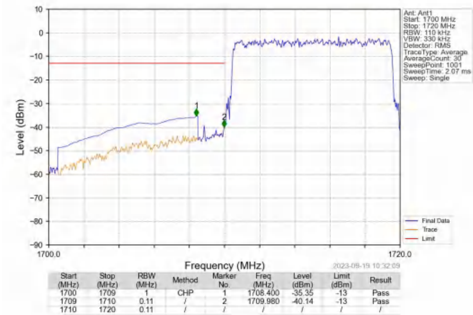
Band4_10MHz_16QAM_LCH_1715MHz_RB_50_0_NTNV
