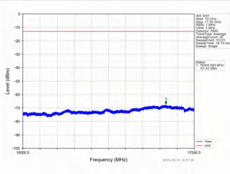
Band4_5MHz_16QAM_HCH_1752.5MHz_RB_1_0_NTNV
