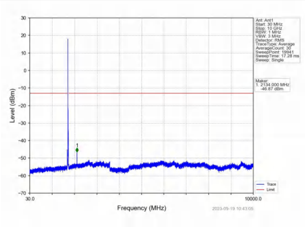
Band4_15MHz_16QAM_MCH_1732.5MHz_RB_1_0_NTNV
