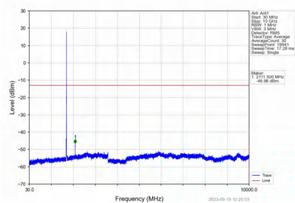
Band4_5MHz_16QAM_LCH_1712.5MHz_RB_1_0_NTNV
