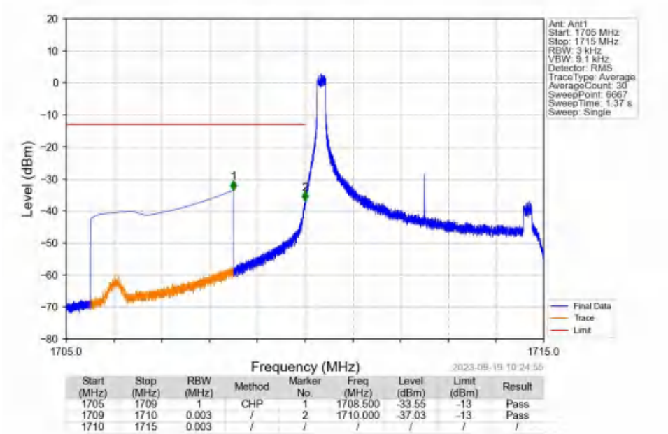
Band4_5MHz_16QAM_LCH_1712.5MHz_RB_1_0_NTNV
