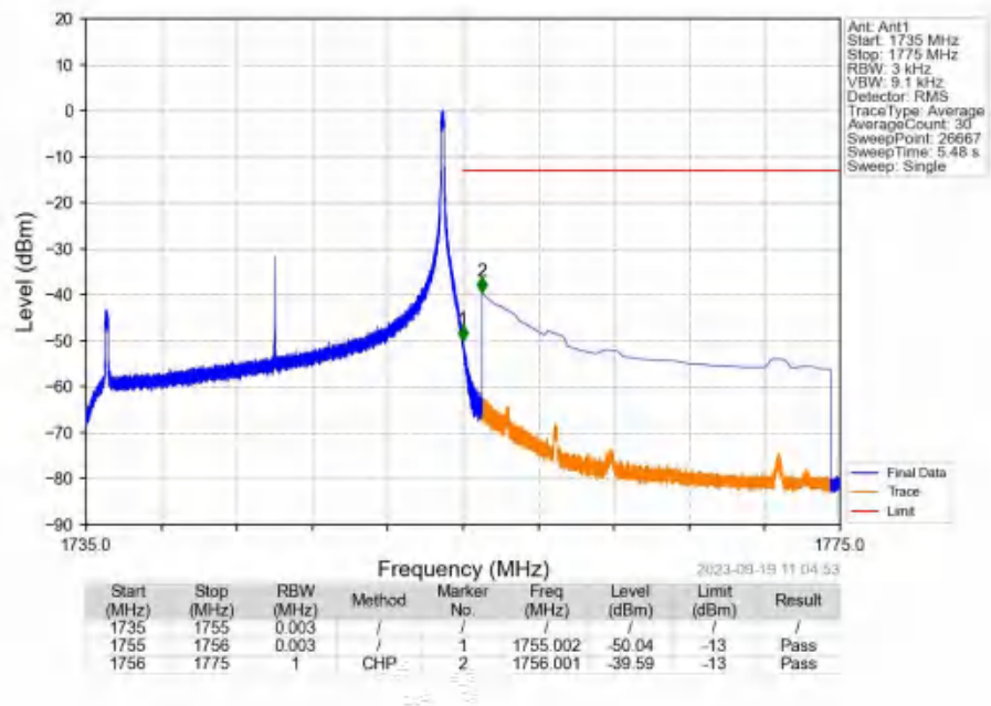
Band4_20MHz_16QAM_HCH_1745MHz_RB_100_0_NTNV
