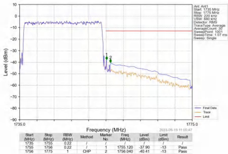
Band4_20MHz_16QAM_HCH_1745MHz_RB_100_0_NTNV
