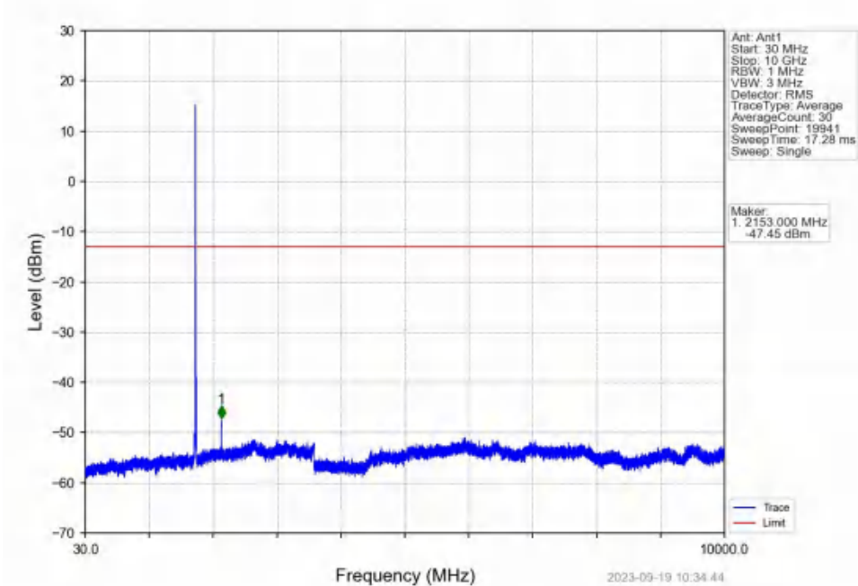
Band4_10MHz_16QAM_HCH_1750MHz_RB_1_0_NTNV
