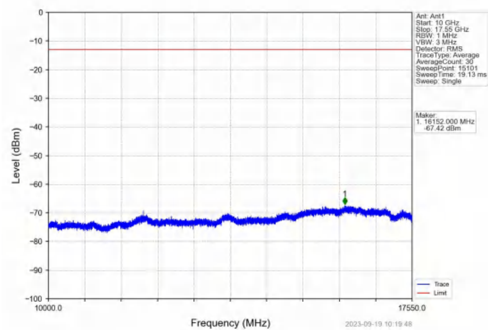
Band4_3MHz_QPSK_LCH_1711.5MHz_RB_15_0_NTNV
