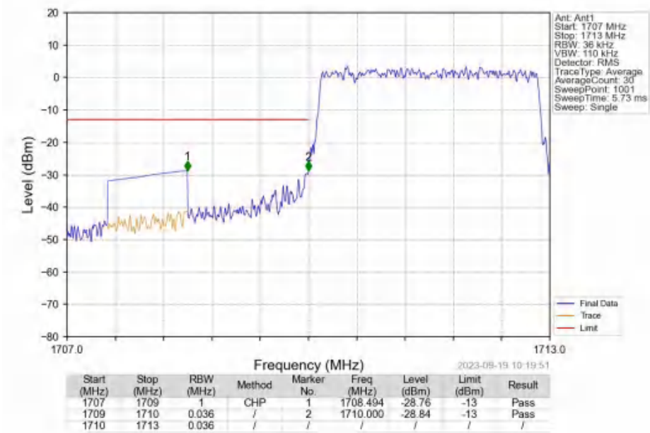
Band4_3MHz_QPSK_LCH_1711.5MHz_RB_15_0_NTNV
