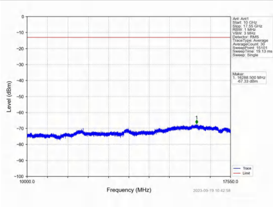
Band4_15MHz_QPSK_MCH_1732.5MHz_RB_1_0_NTNV
