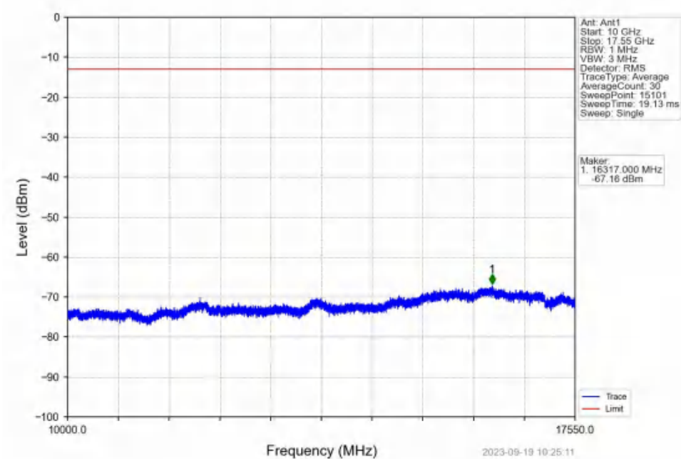
Band4_5MHz_16QAM_LCH_1712.5MHz_RB_25_0_NTNV
