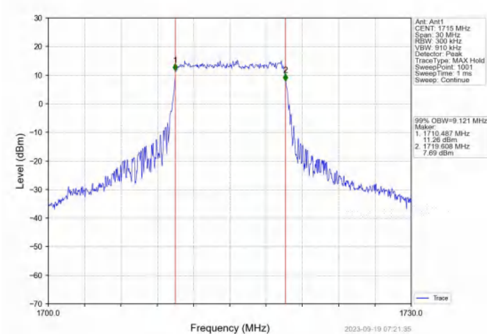
Band4_10MHz_16QAM_LCH_1715MHz_RB_50_0_NTNV
