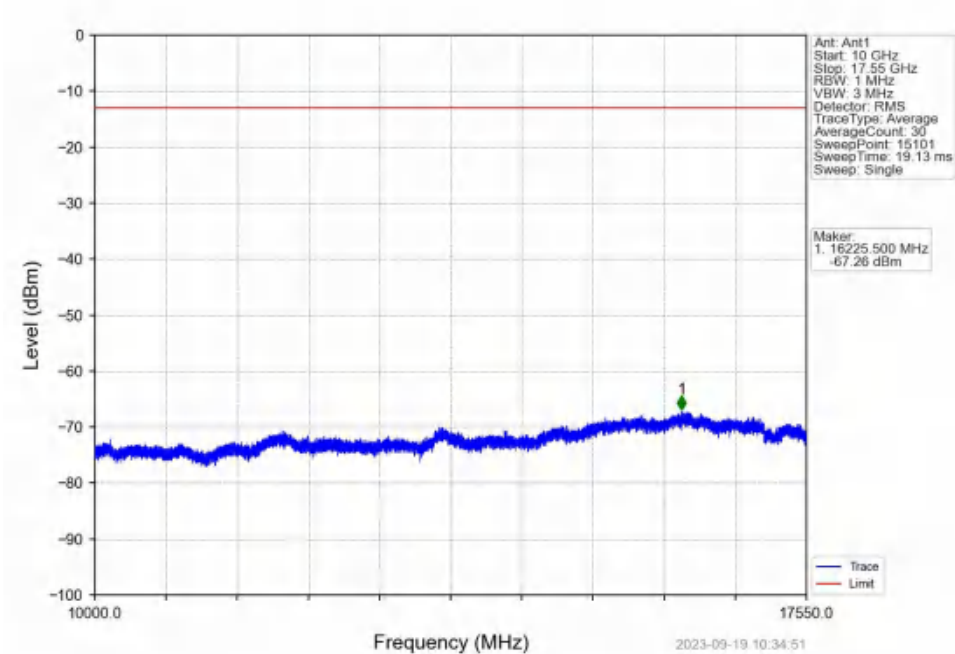
Band4_10MHz_16QAM_HCH_1750MHz_RB_1_0_NTNV
