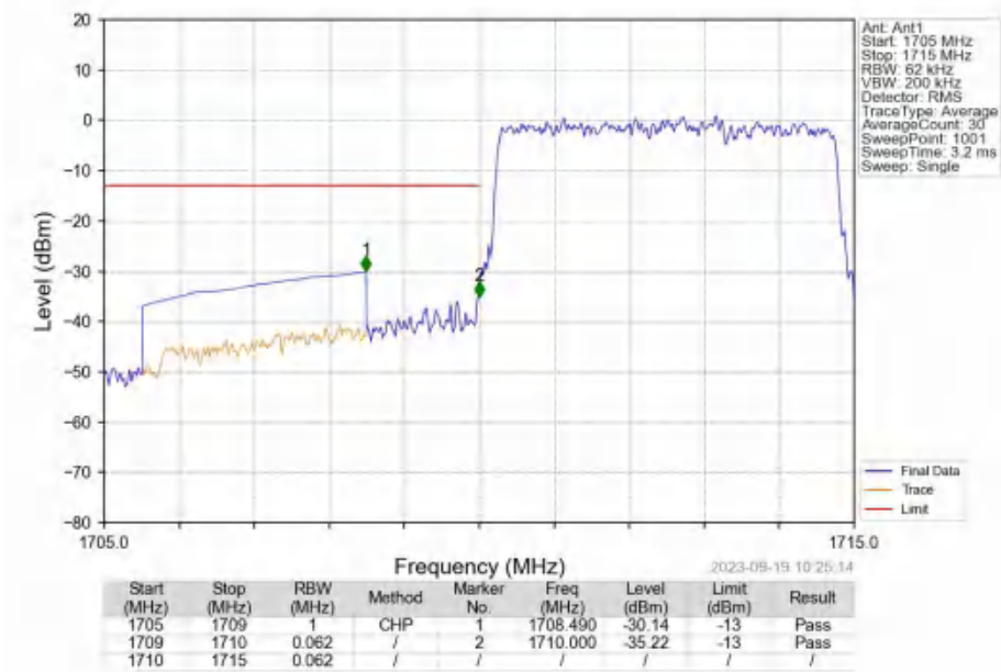
Band4_5MHz_16QAM_LCH_1712.5MHz_RB_25_0_NTNV
