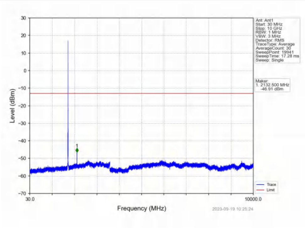
Band4_5MHz_QPSK_MCH_1732.5MHz_RB_1_0_NTNV
