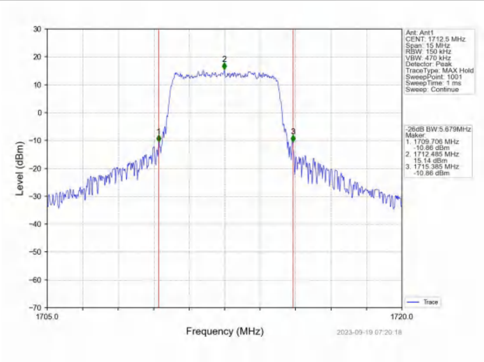
Band4_5MHz_16QAM_LCH_1712.5MHz_RB_25_0_NTNV
