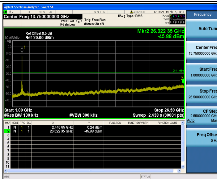
802.11n(HT40)_2452_0~Reference
