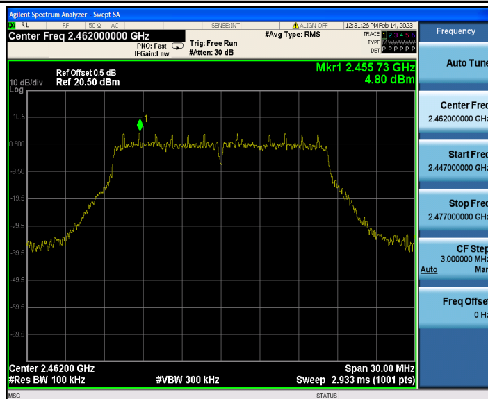
802.11g_2462_30~1000
