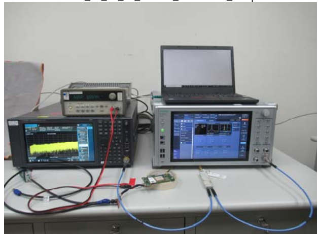
FCC_22_24_27_Cat-M1_Conducted_setup
