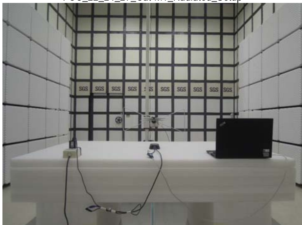
FCC_22_24_27_Cat-M1_Radiated_Setup
