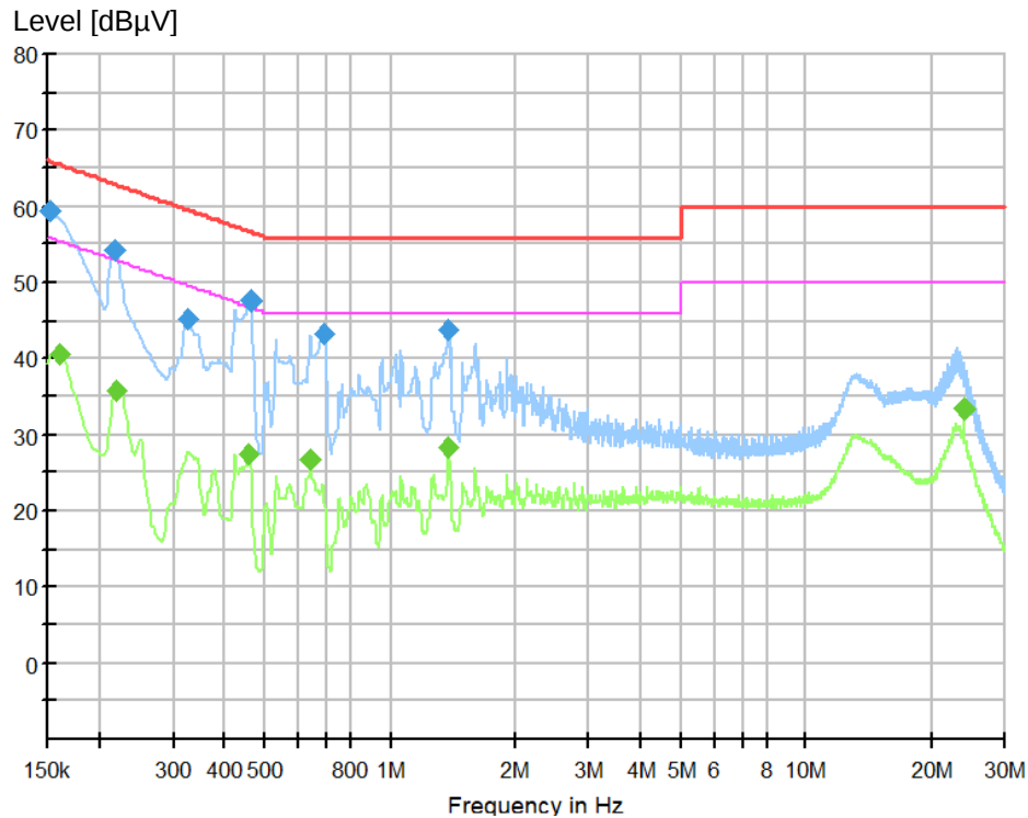
Figure 6: Spectral Diagrams, Conducted Emission, 150 kHz – 30 MHz, N on mode 3
