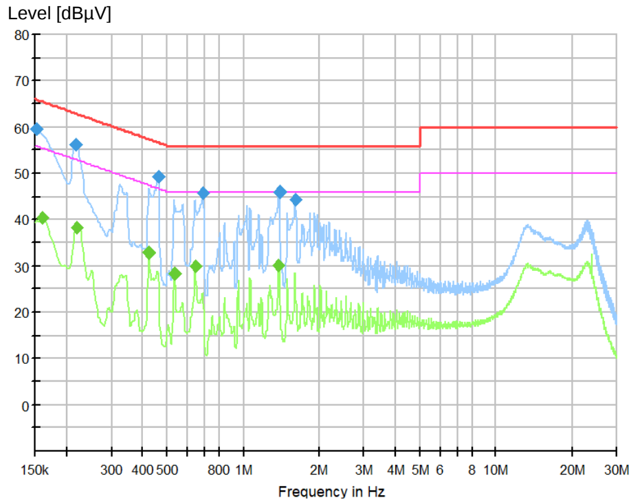
Figure 5: Spectral Diagrams, Conducted Emission, 150 kHz – 30 MHz, L on mode 3
