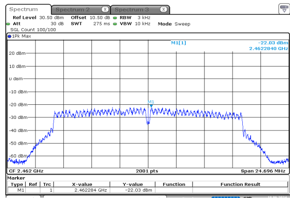
g_2462MHz_Chain 0
