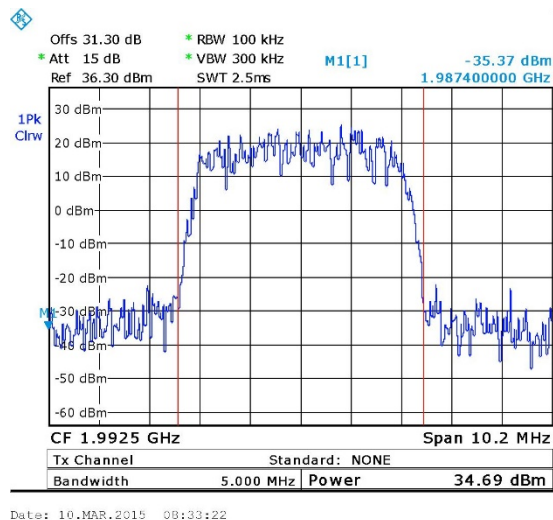
Figure 16. — W-CDMA - 1992.50 MHz
