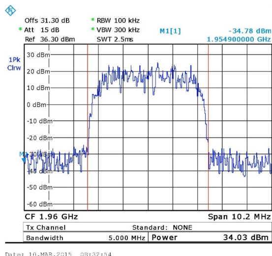
Figure 15. — W-CDMA - 1960.00 MHz
