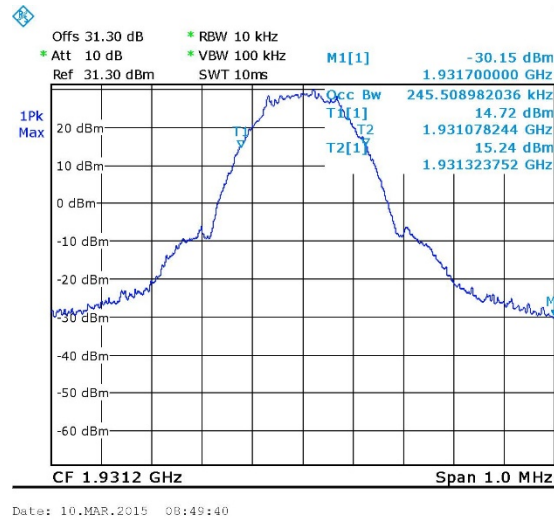
Figure 25. — GSM - Input 1931.20 MHz
