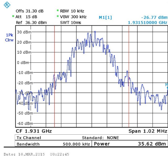
Figure 11. — GSM - 1931.20 MHz
