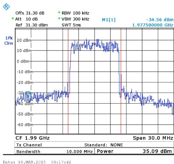
Figure 10. — LTE 64QAM 1990.00 MHz
