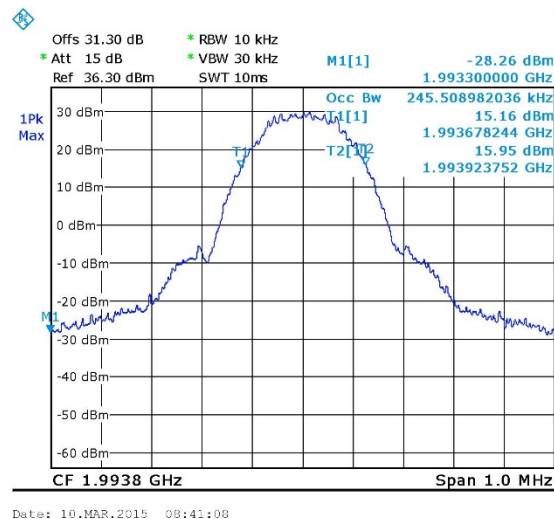
Figure 30. — GSM - Output 1993.80 MHz
