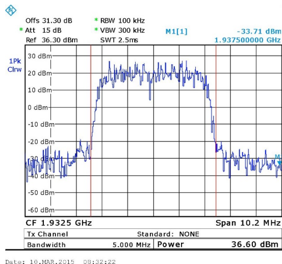
Figure 14. — W-CDMA - 1932.50 MHz
