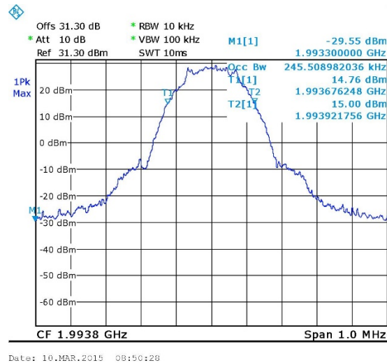
Figure 29. — GSM - Input 1993.80 MHz
