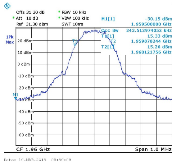
Figure 27. — GSM - Input 1960.00 MHz
