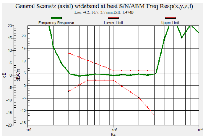
Fig 7.1 LTE Band 13
