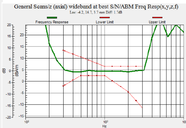
Fig 7.2 LTE Band 13
