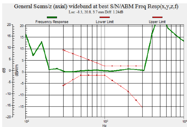
Fig. 7.5 LTE Band 13
