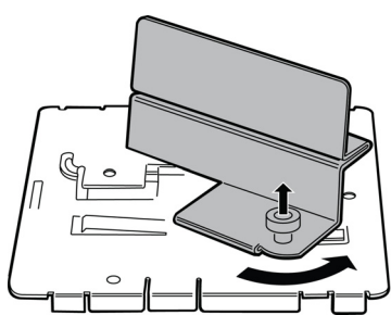
Figure 6 Attaching the adapter to the main bracket
