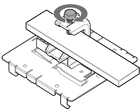
Figure 7 Attaching the beam clamp on a beam
