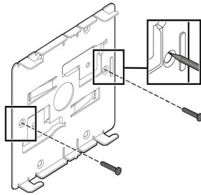
Figure 3 AP-7632i Main Bracket
