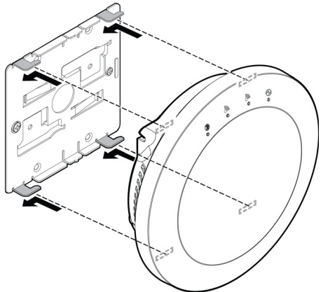
Figure 4 Attaching the AP to a Wall using the Main Bracket
