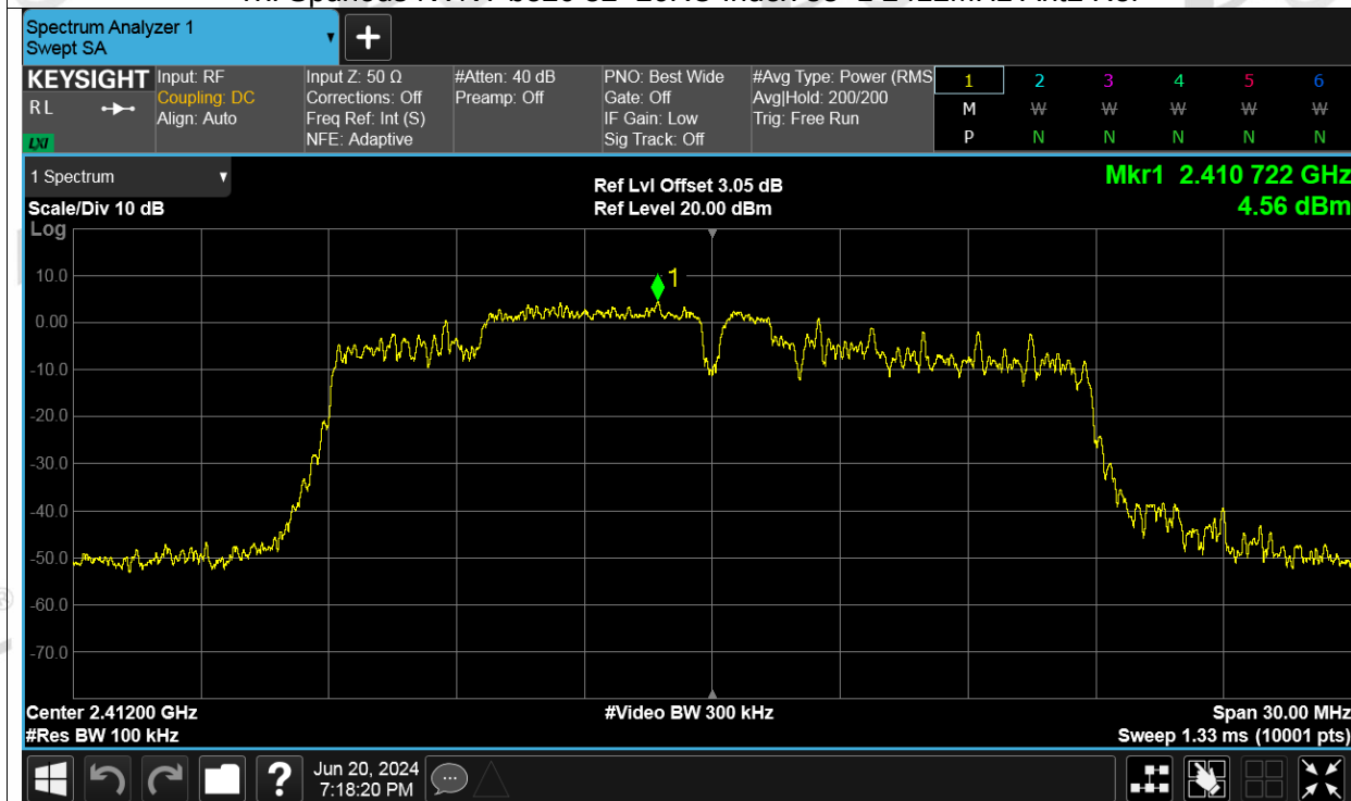
Tx. Spurious NVNT be20 52+26RU Index 38+1 2412MHz Ant2 Emission
