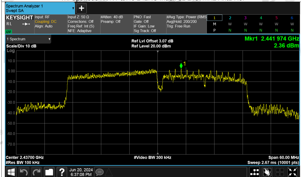
Tx. Spurious NVNT ax40 242RU Index 61 2437MHz Ant1 Emission
