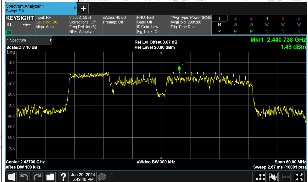
Tx. Spurious NVNT ax40 106RU Index 53 2437MHz Ant1 Emission
