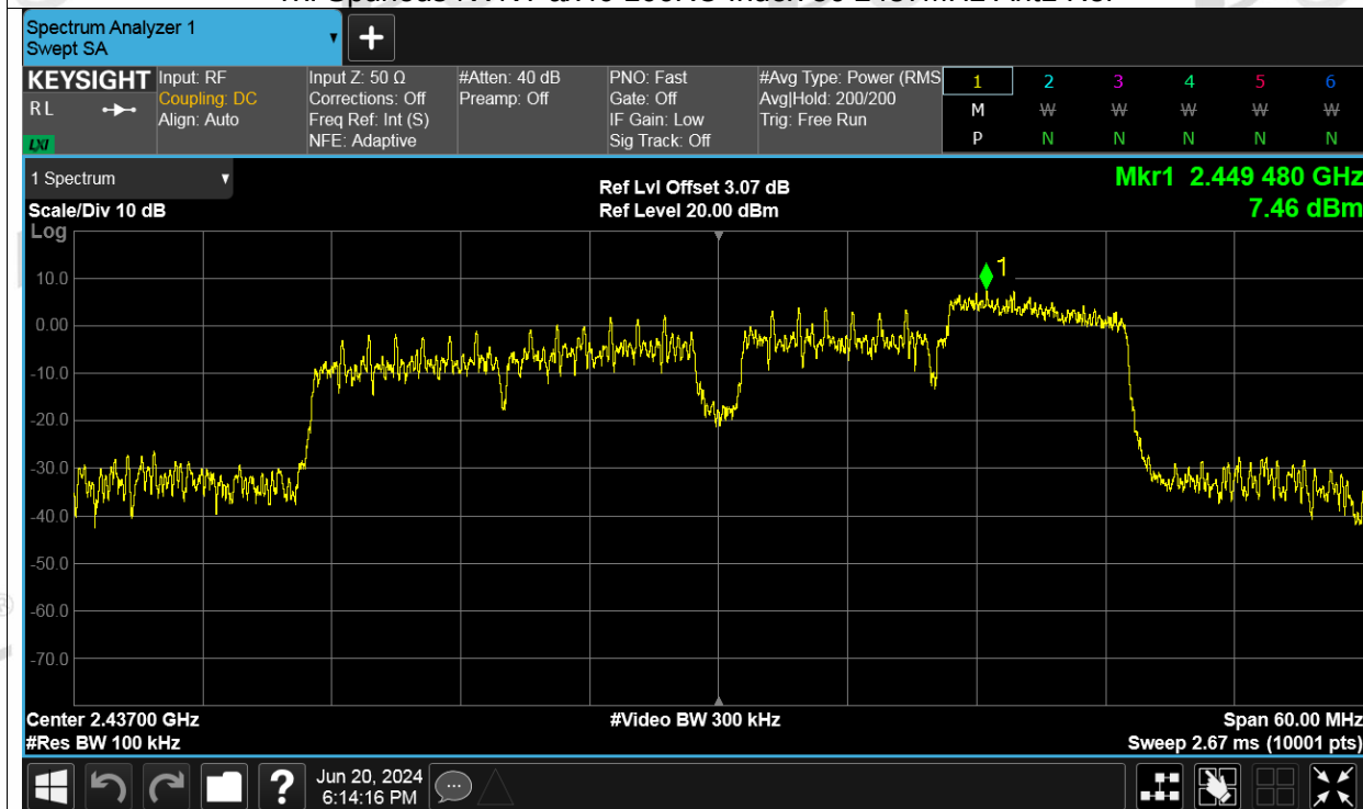
Tx. Spurious NVNT ax40 106RU Index 56 2437MHz Ant1 Emission
