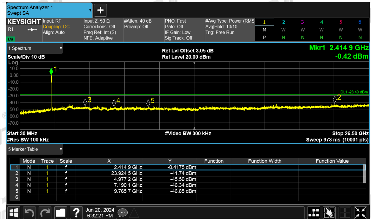
Tx. Spurious NVNT ax40 242RU Index 61 2437MHz Ant1 Ref
