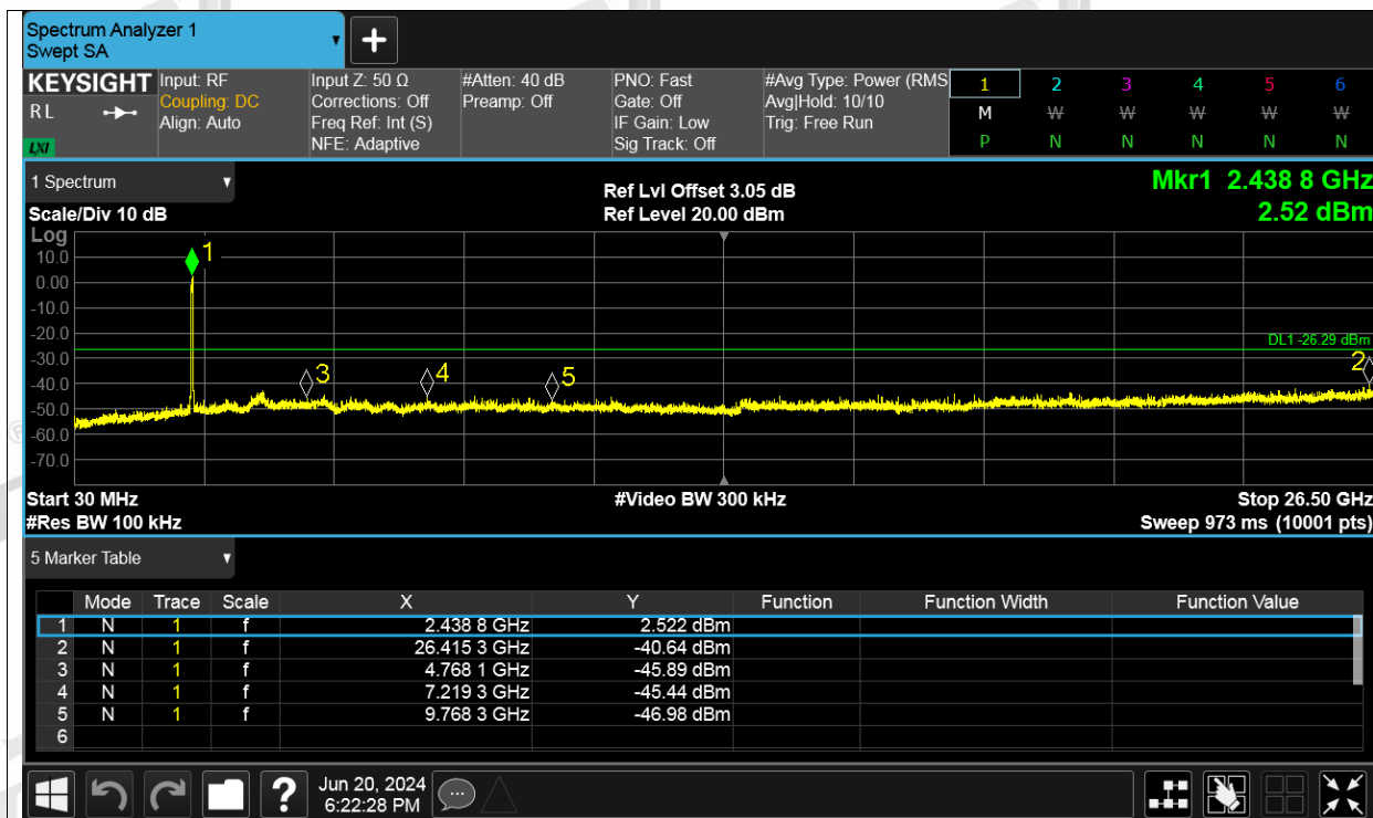
Tx. Spurious NVNT ax40 106RU Index 56 2437MHz Ant1 Ref
