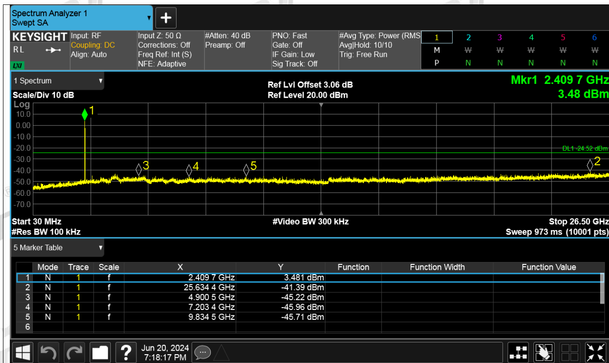
Tx. Spurious NVNT be20 52+26RU Index 38+1 2412MHz Ant2 Ref
