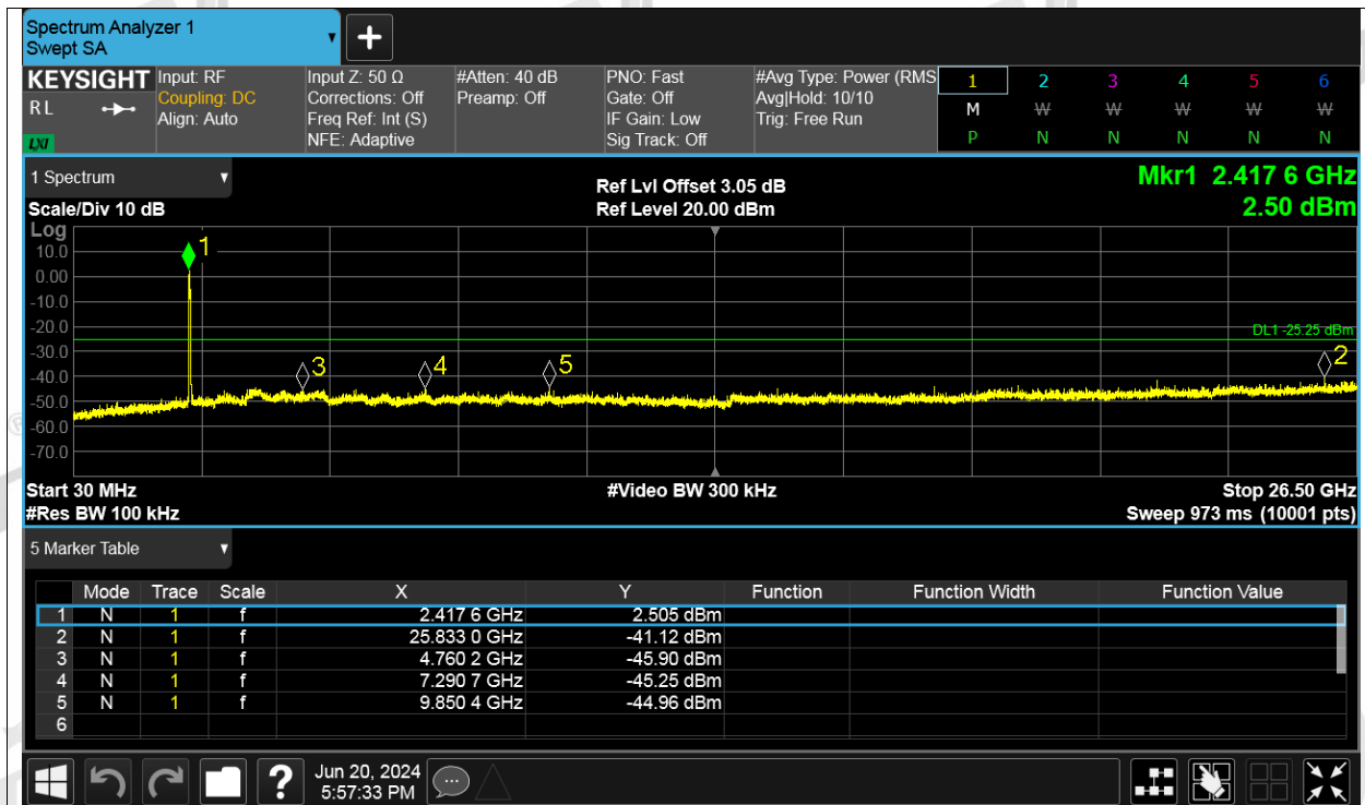
Tx. Spurious NVNT ax40 106RU Index 54 2437MHz Ant1 Ref
