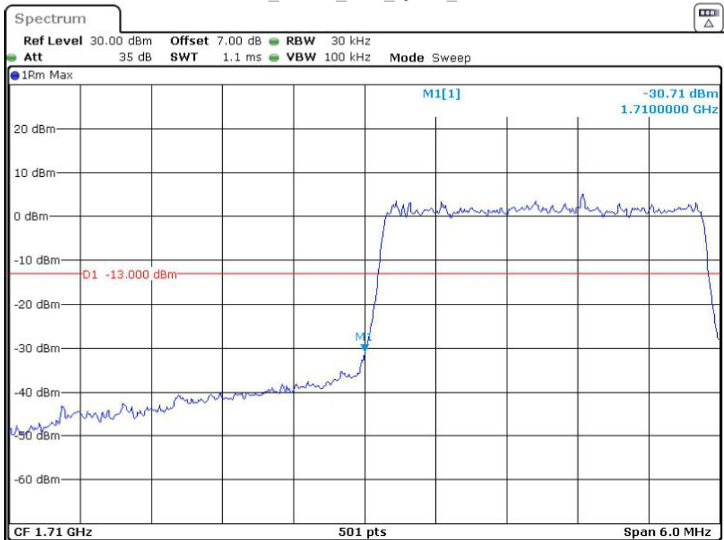
Band 66_3 MHz_Low_QPSK_RB15#0
