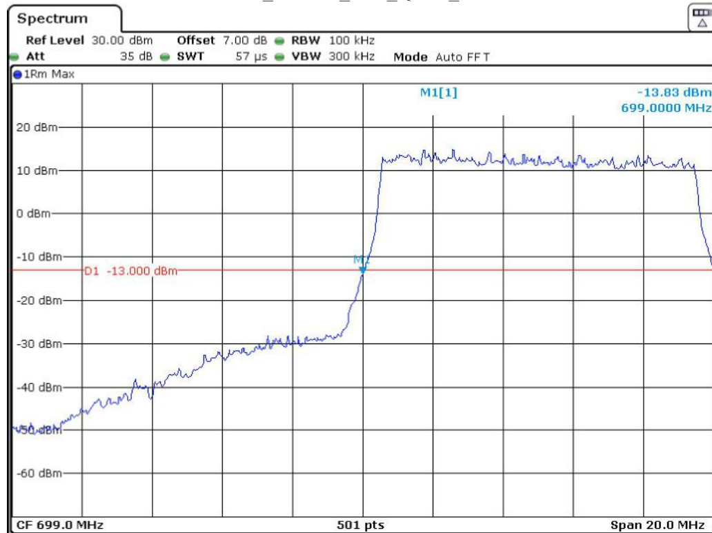
Band 12_10 MHz_Low_QPSK_RB50#0
