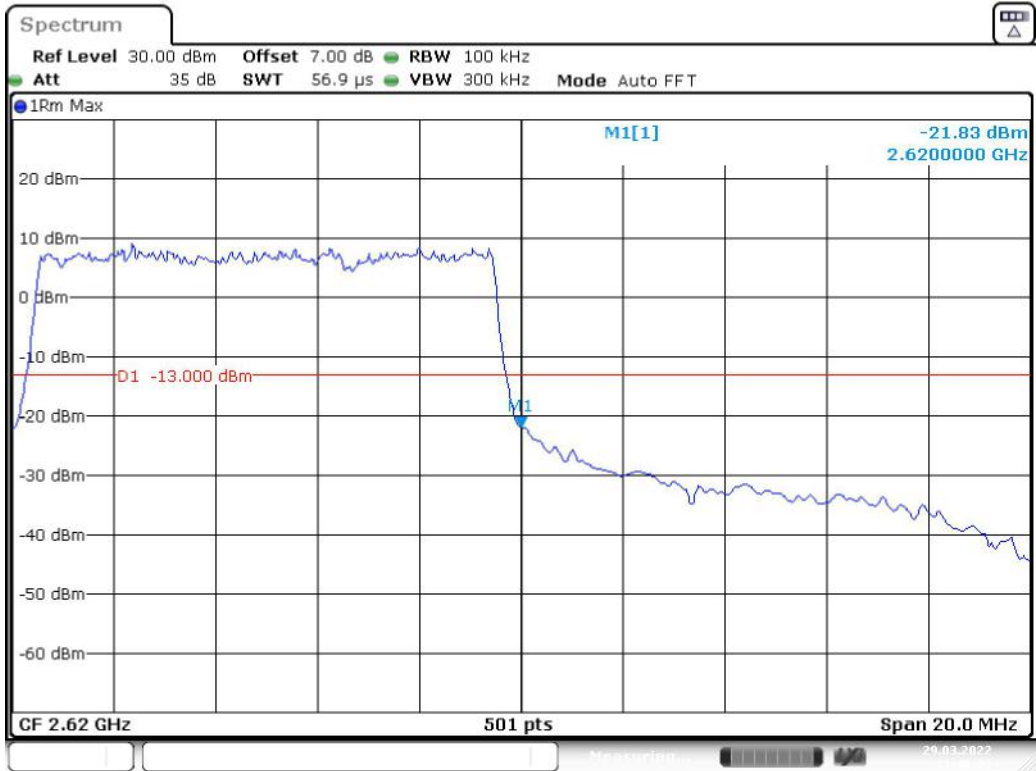
Band 38_10 MHz_High_QPSK_RB50#0
