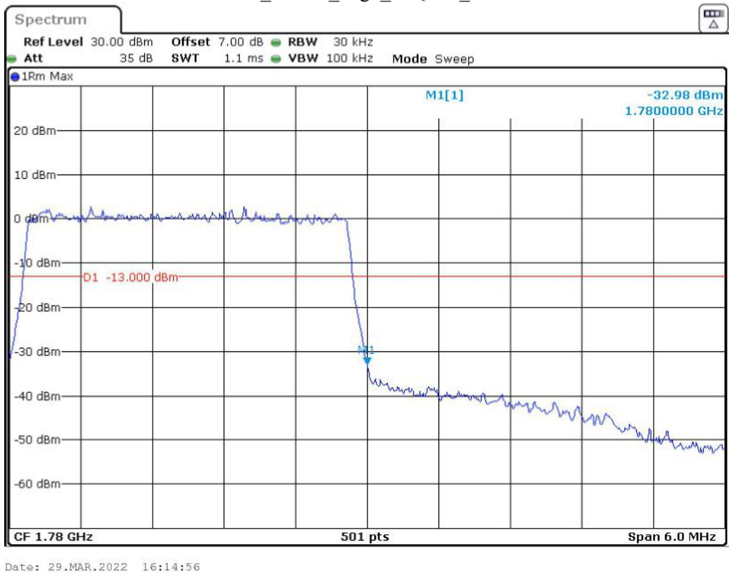
Band 66_3 MHz_High_16QAM_RB15#0
