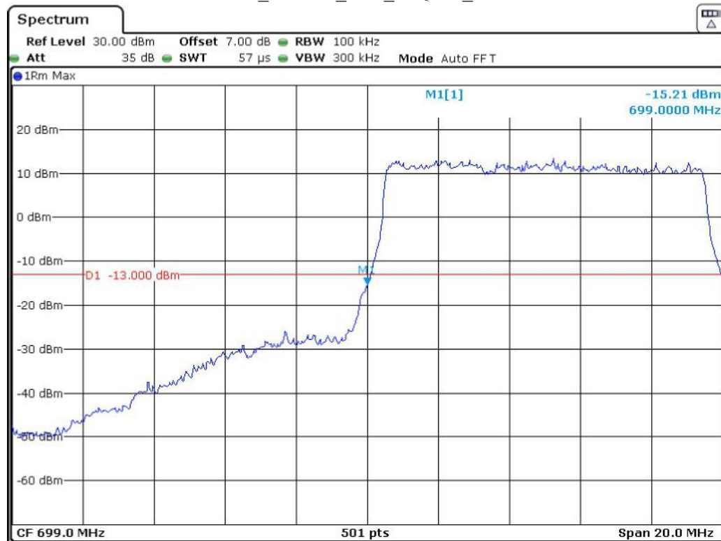
Band 12_10 MHz_Low_16QAM_RB50#0
