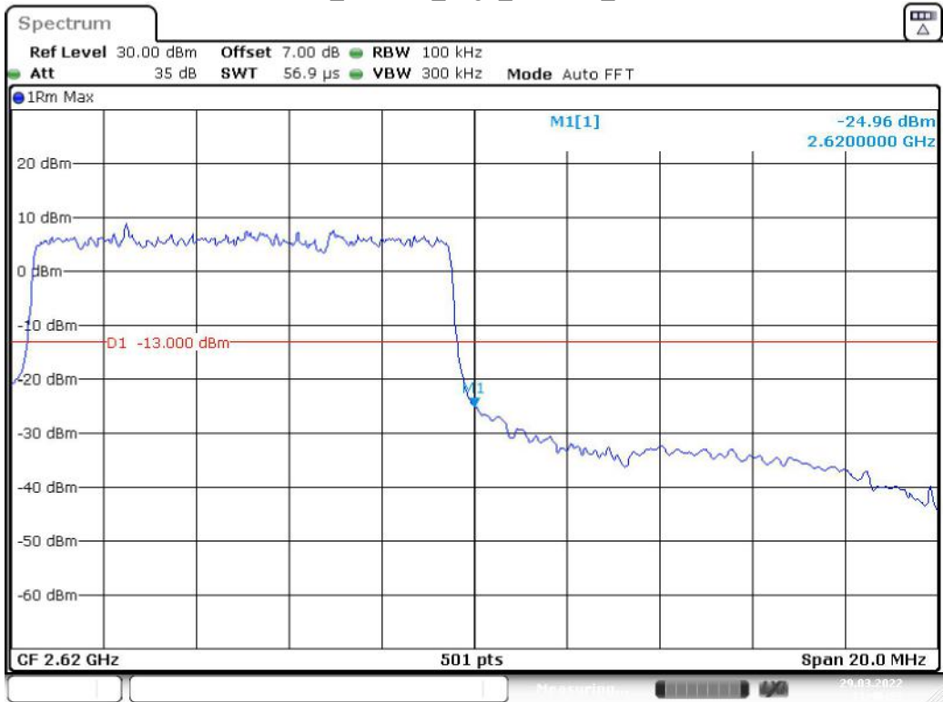
Band 38_10 MHz_High_16QAM_RB50#0
