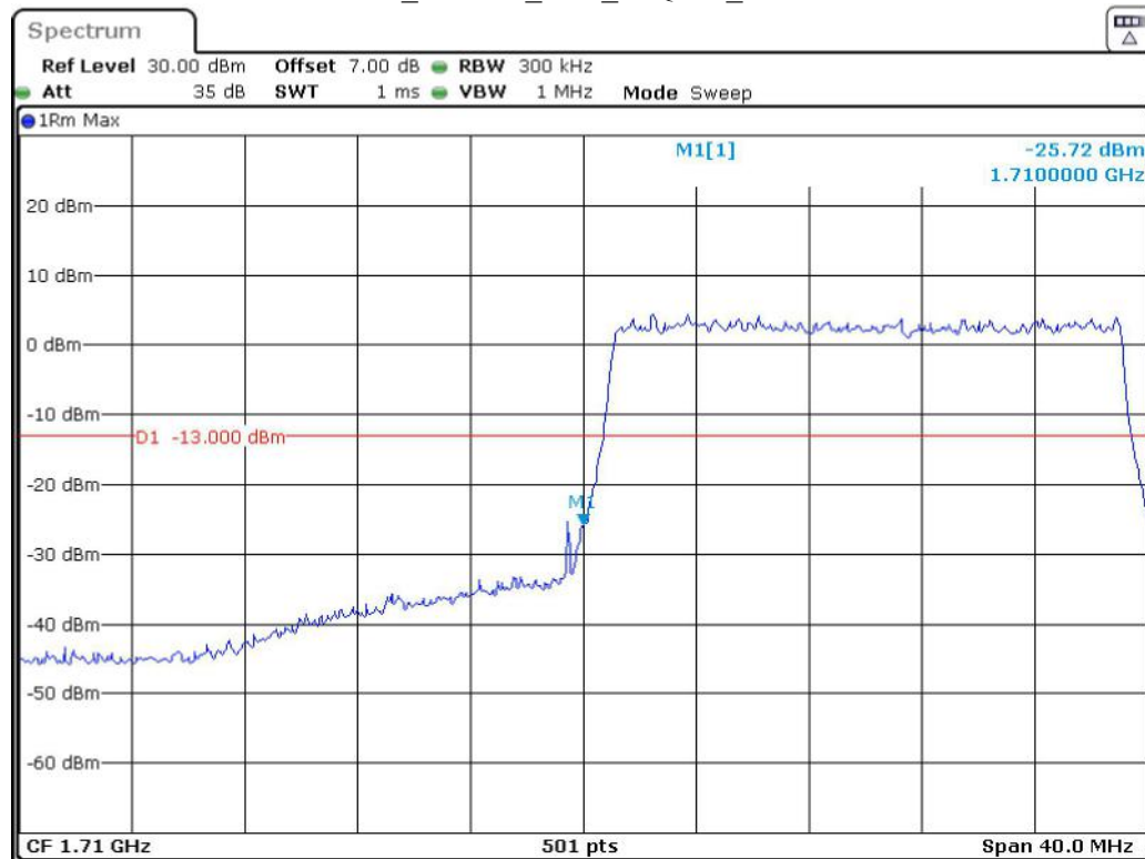
Band 66_20 MHz_Low_16QAM_RB100#0
