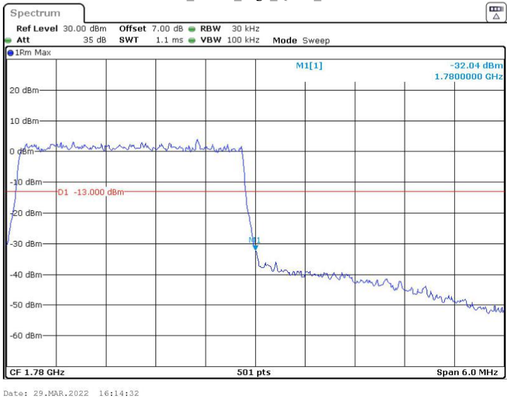
Band 66_3 MHz_High_QPSK_RB15#0
