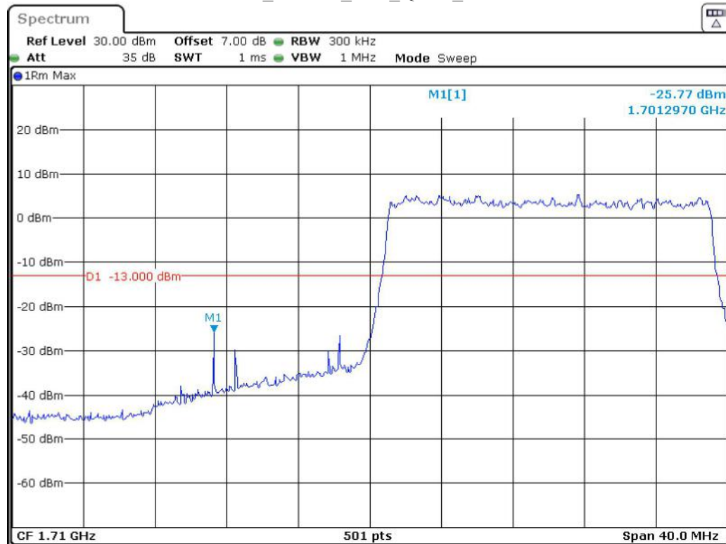
Band 66_20 MHz_Low_QPSK_RB100#0
