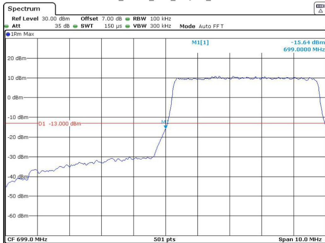
Band 12_5 MHz_Low_16QAM_RB25#0
