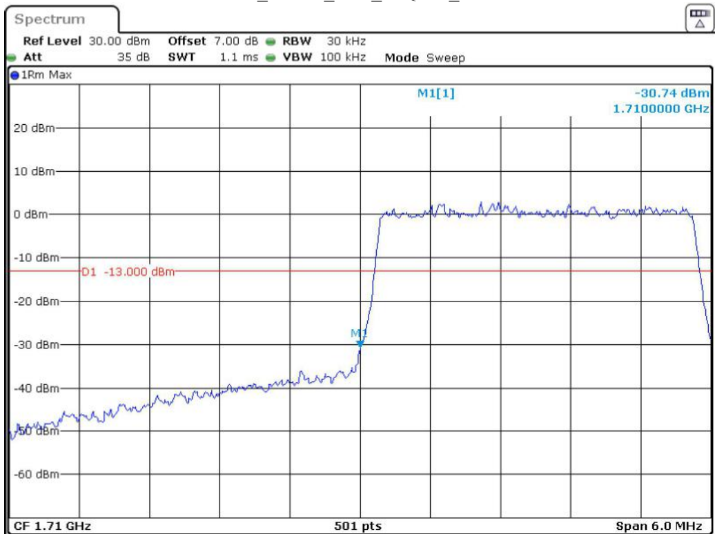
Band 66_3 MHz_Low_16QAM_RB15#0
