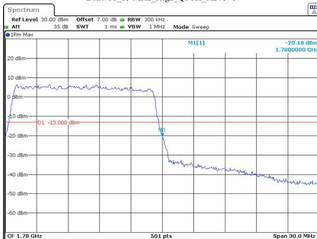
Band 66_15 MHz_High_QPSK_RB75#0
