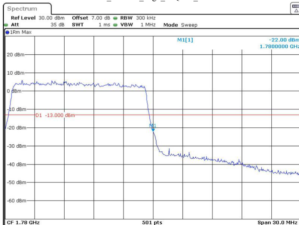
Band 66_15 MHz_High_16QAM_RB75#0
