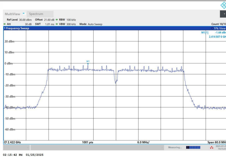
11N40SISO_Ant1_2422_30~1000
