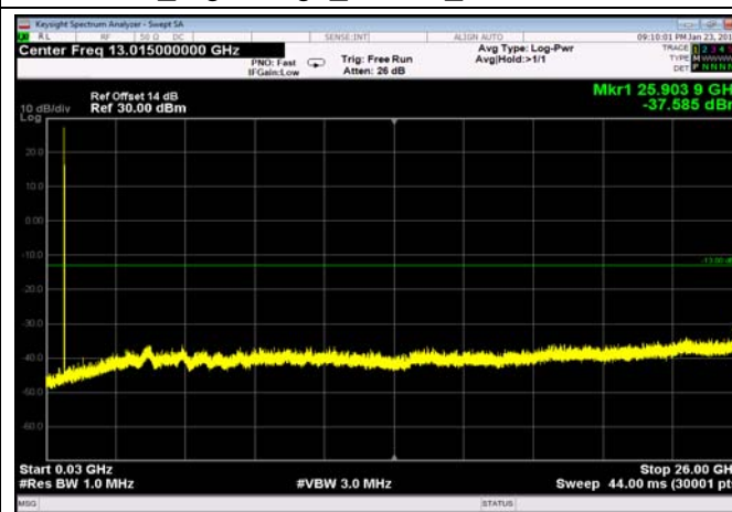
FDD12_HighRange_5MHz_30MHz~26GHz
