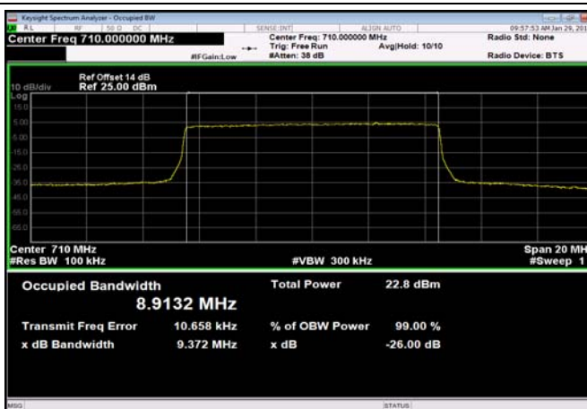
FDD17_MidRange_10_710_QPSK
