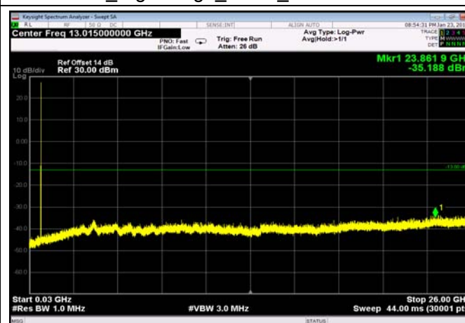
FDD12_HighRange_5MHz_30MHz~26GHz
