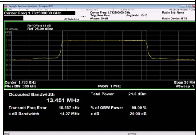
FDD04_MidRange_20MHz_1732.5MHz
