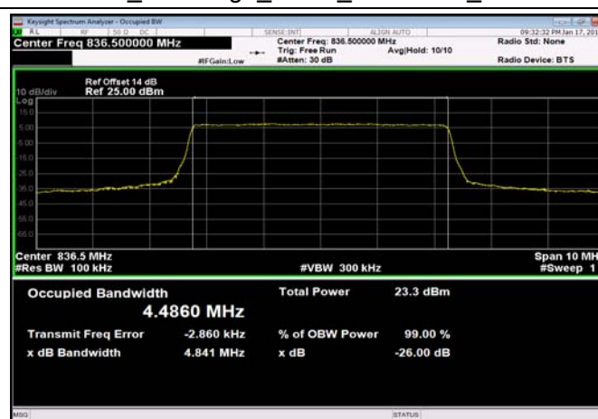
FDD05_MidRange_5MHz_836.5MHz_QPSK
