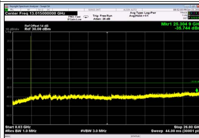
FDD12_HighRange_10MHz_30MHz~26GHz
