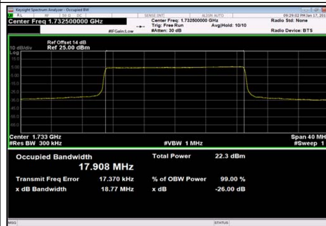
FDD04_MidRange_20MHz_1732.5MHz QPSK
